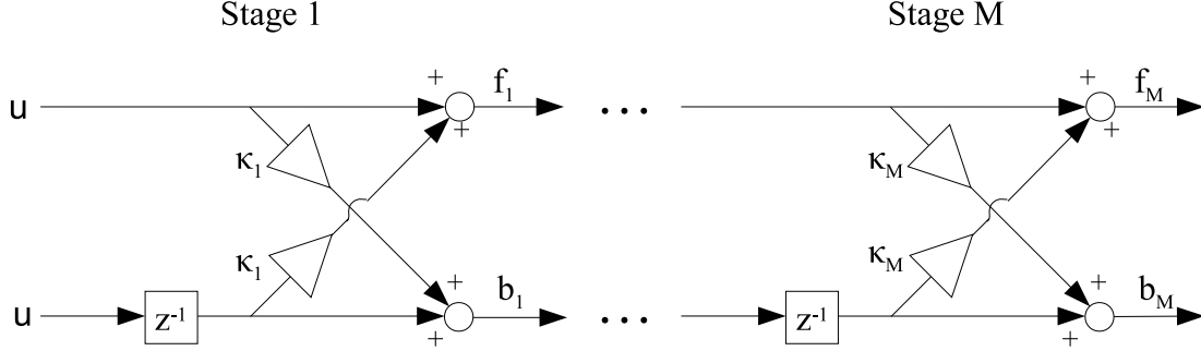
Figure 2.11: A lattice filter consists of a cascade M stages with an identical structure. Each stage is characterized by its reflection coefficient, \kappa_m . The name lattice filter comes from the lattice-like appearance of the stages.
