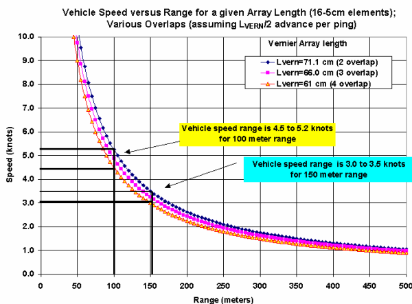
Figure 1. Range-Speed Envelope for SAS12
