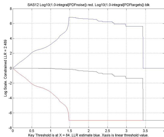
Figure 18: Log Pd, Log Pfa, and LLR for the five SAS12 images considered.
