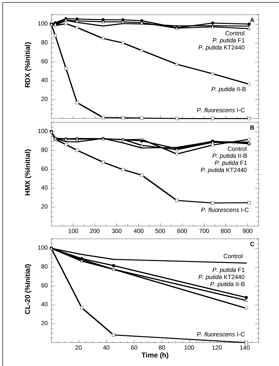
Figure 2. Degradation of A) RDX, B) HMX, and c) CL-20 by pure cultures of Pseudomonas spp. under anaerobic conditions. Sterile control (—); P. putida II-B (O); P. fluorescens I-C (□); P. putida F1 (●); P. putida KT2440 (△). Datapoints represent average of two replicate cultures. Note difference in x-axis scales.
