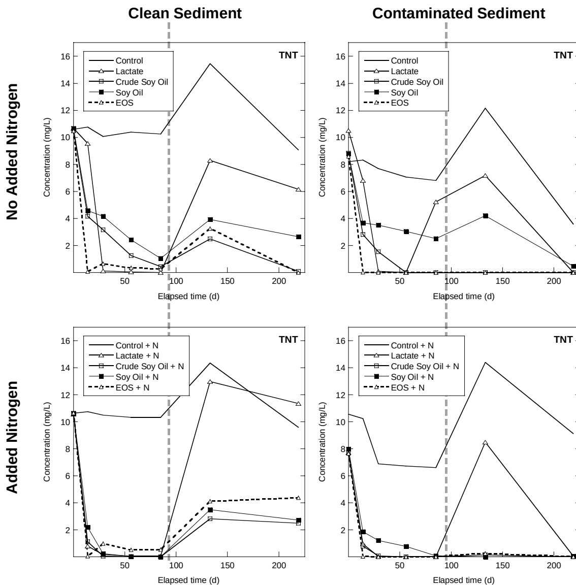
Figure 3.1-2. Degradation of TNT in WVO microcosm enrichments. The vertical dashed line indicates when the microcosms were respiked with the explosive and/or other amendments.
