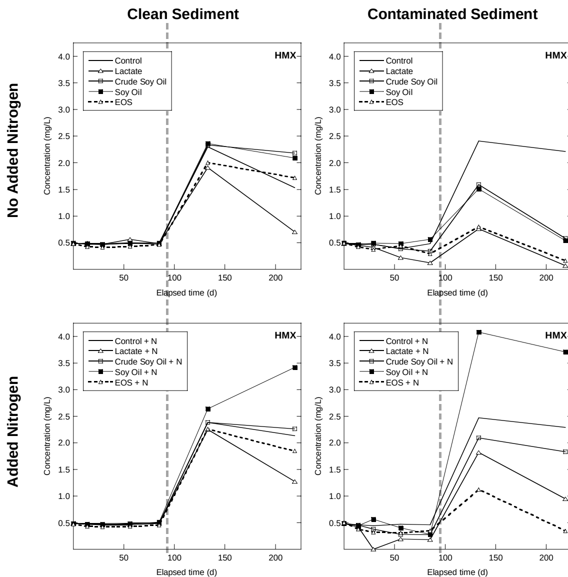
Figure 3.1-4. Degradation of HMX in WVOW microcosm enrichments. The vertical dashed line indicates when the microcosms were respired with the explosive and/or other amendments.
