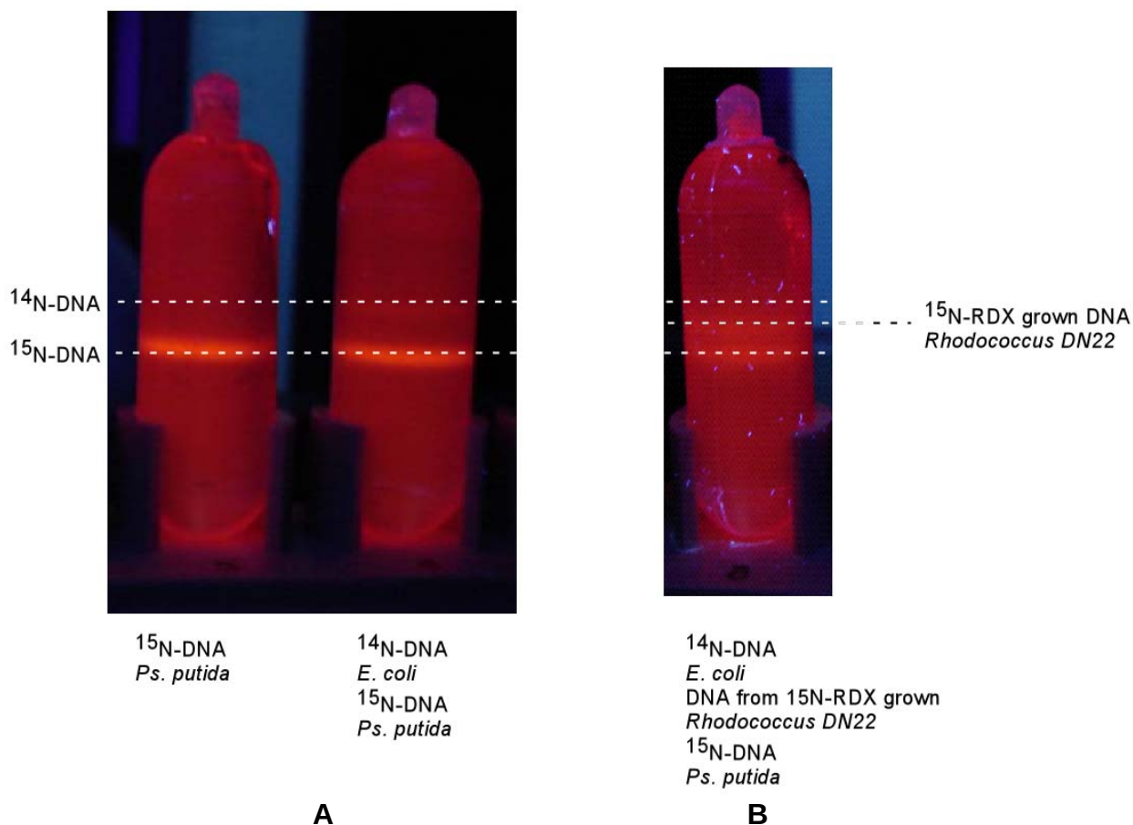
Figure 4.1-2. Separation of stable ^{15}\text{N} isotope-labelled DNA by ultracentrifugation. A) Separation of ^{14}\text{N} -DNA of E. coli from ^{15}\text{N} -DNA of Ps. putida after ultracentrifugation. The upper band is ^{14}\text{N} -DNA and lower band is ^{15}\text{N} -DNA. (right) The band of ^{15}\text{N} -DNA of Rhodococcus sp. DN22 (after degrading ring- ^{15}\text{N} -labelled RDX) located between that of ^{14}\text{N} -DNA and ^{15}\text{N} -DNA controls.
