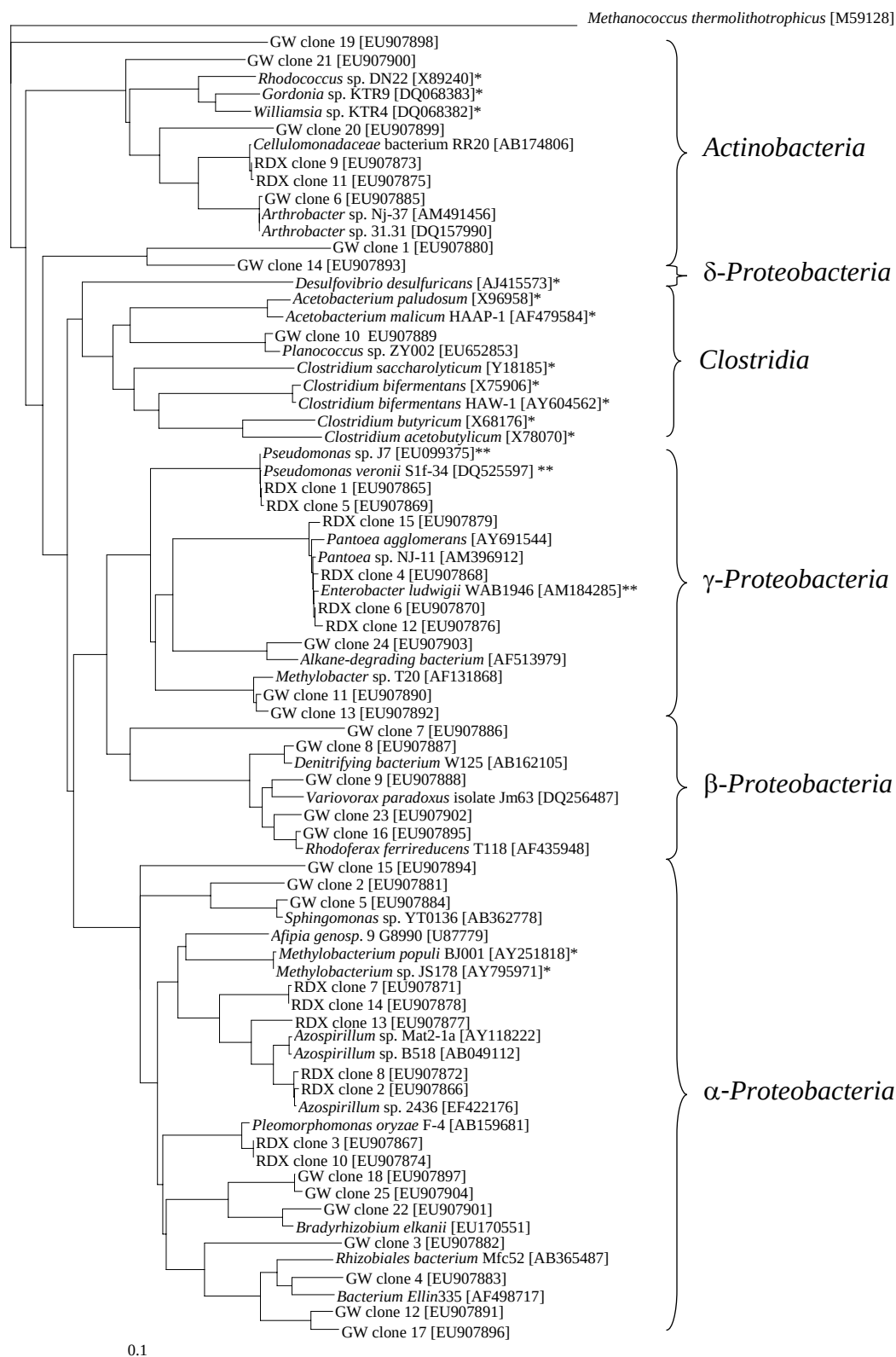
Figure 3. Phylogenetic analysis of cloned bacterial 16S rRNA genes from ^{15}\text{N} -DNA fraction.
