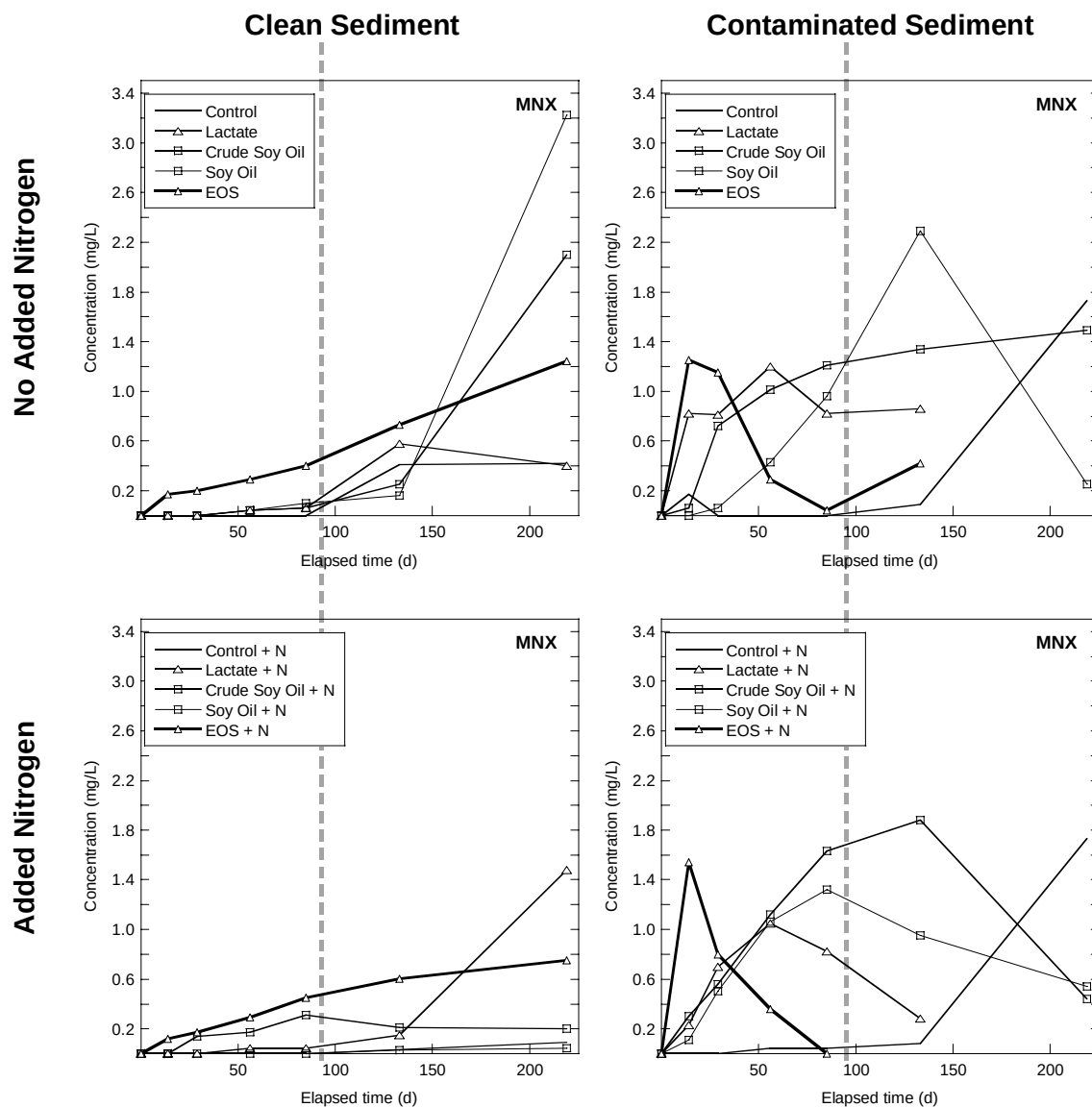
Figure 3.1-5. Concentrations of MNX in WVO microcosm enrichments. The vertical dashed line indicates when the microcosms were respiked with the explosive and/or other amendments.
