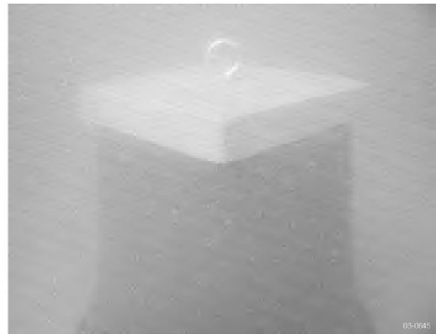
Fig. 20. Left: Plot of autonomous raster search of a test field during AUV Fest 2001. Right: Located target image. The target was detected using the bumper and the camera image was compressed 50:1 using the UCSD-developed compression codes. The image was then transmitted at 1200 baud using the Benthos ATM885 telesonar modem to an RF buoy, which relayed the image to the Operator Control Station (OCS), where it was decompressed and displayed.
