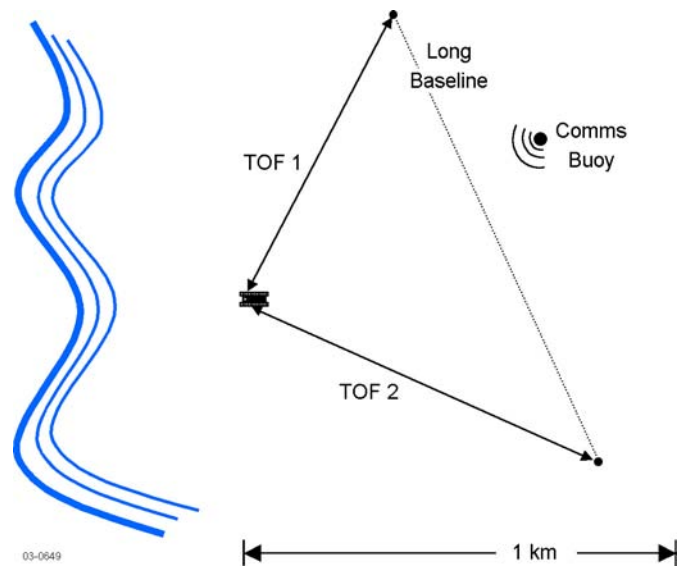
Fig. 24. Navigation/communication sonar deployment.
