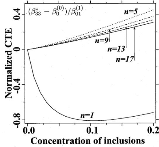
Figure 2.49: Normalized CTE (\beta_{33}^* - \beta_0^{(0)})/\beta_{01}^{(1)} vs c^{(1)} for the different inclusion number n = 1, 5, 9, 13, 17 in the clusters.
