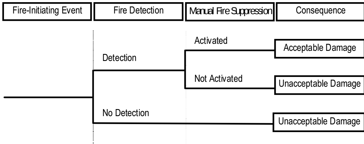
Figure 3—Fire Event Tree for Areas with Manual Fire Suppression System
