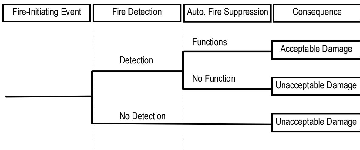
Figure 2—Fire Event Tree for Areas with Automatic Fire Suppression System
