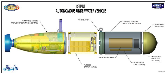
Figure 1. RELIANT/SAS21 System
