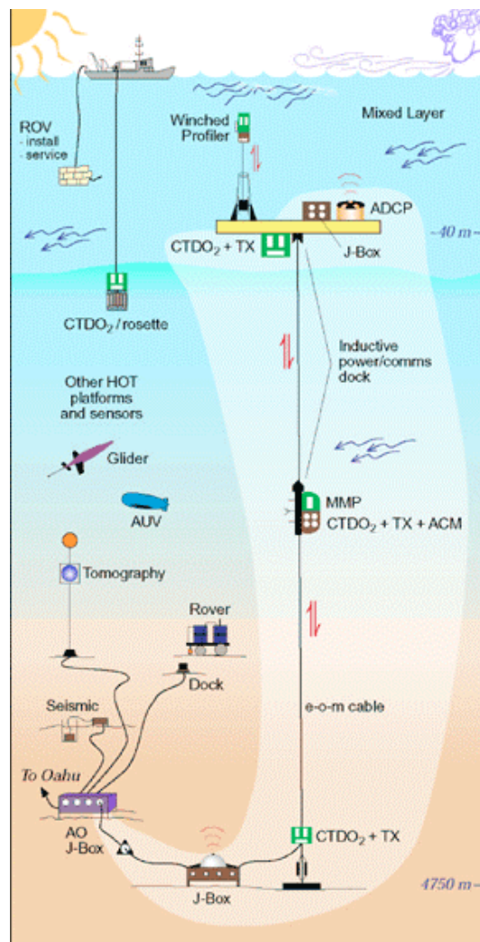
Figure 2. Schematic of a real-time cabled profiling mooring. This moored sensor network will consist of an instrumented profiler that will move between near-surface and abyssal fixed sensors under program control (figure courtesy of Bruce Howe, UW).
