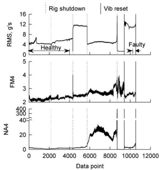
Figure B5. Set 5 vibration fault detection data.
