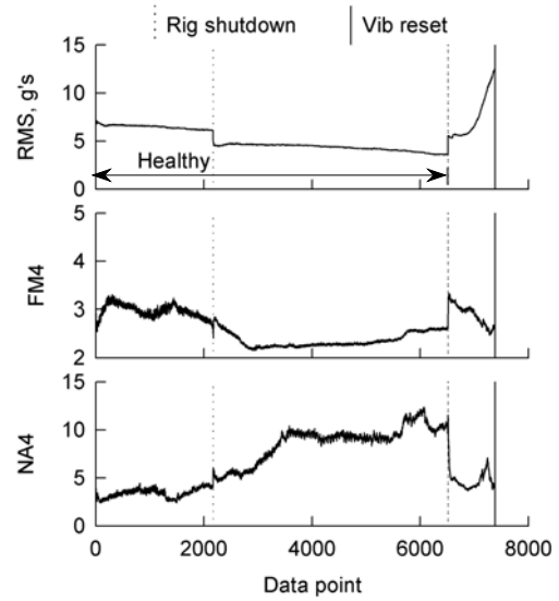
Figure B11. Set 11 vibration fault detection data.
