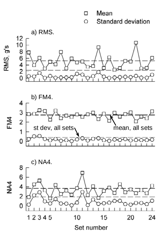
Figure 5. Mean and standard deviation statistics for all sets, healthy state condition.
