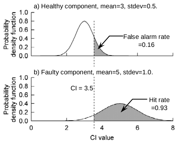
Figure 7. Sample probability density functions.
