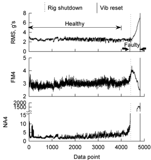
Figure B17. Set 17 vibration fault detection data.
