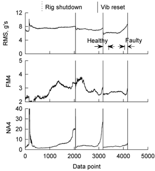
Figure B9. Set 9 vibration fault detection data.
