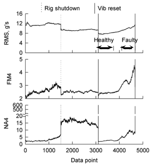
Figure B7. Set 7 vibration fault detection data.
