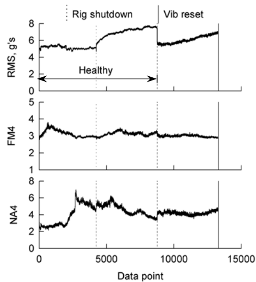
Figure B24. Set 24 vibration fault detection data.
