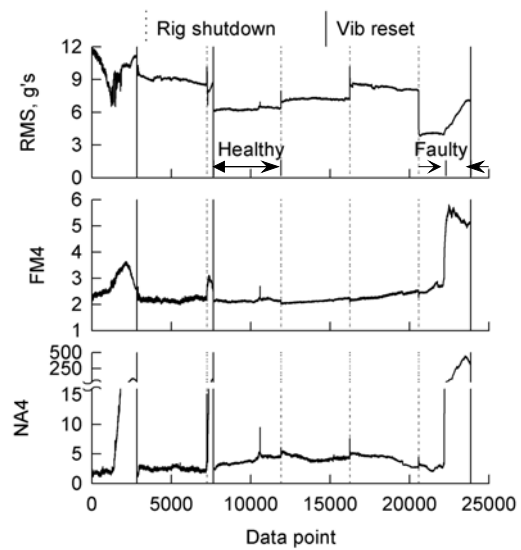
Figure B16. Set 16 vibration fault detection data.
