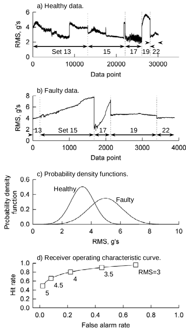
Figure 9. Summary results for RMS condition indicator for macro-pitting, single/few teeth failures.
