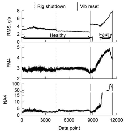
Figure B15. Set 15 vibration fault detection data.
