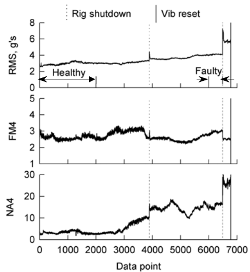
Figure B22. Set 22 vibration fault detection data.
