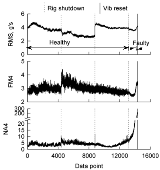
Figure B13. Set 13 vibration fault detection data.
