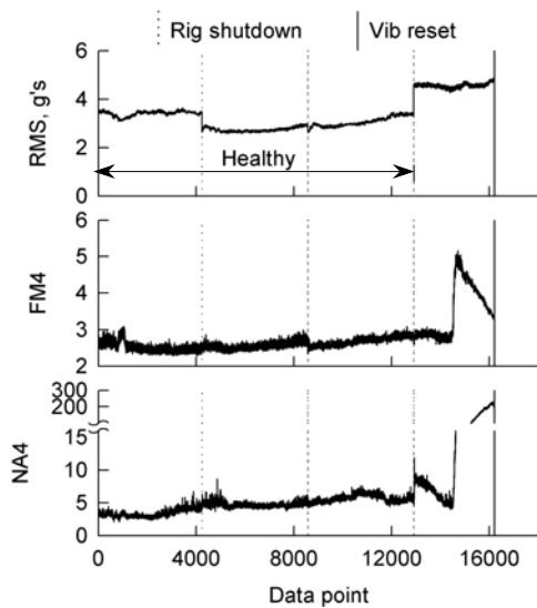
Figure B18. Set 18 vibration fault detection data.
