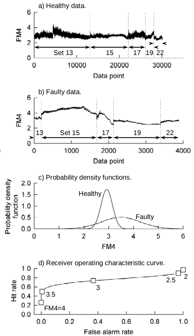
Figure 10. Summary results for FM4 condition indicator for macro-pitting, single/few teeth failures.
