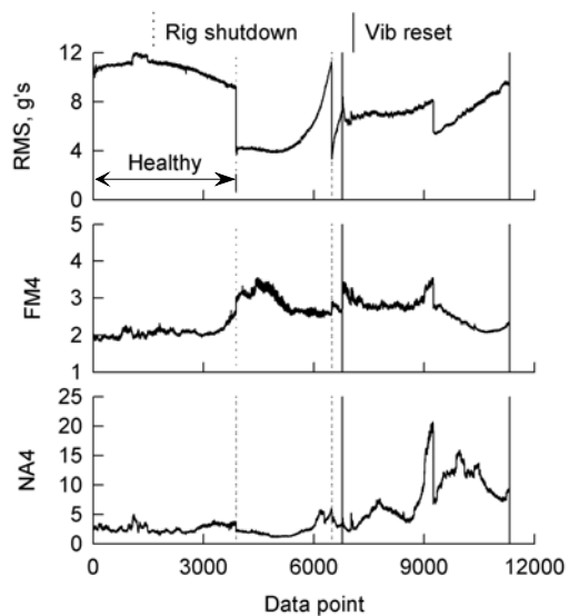
Figure B21. Set 21 vibration fault detection data.
