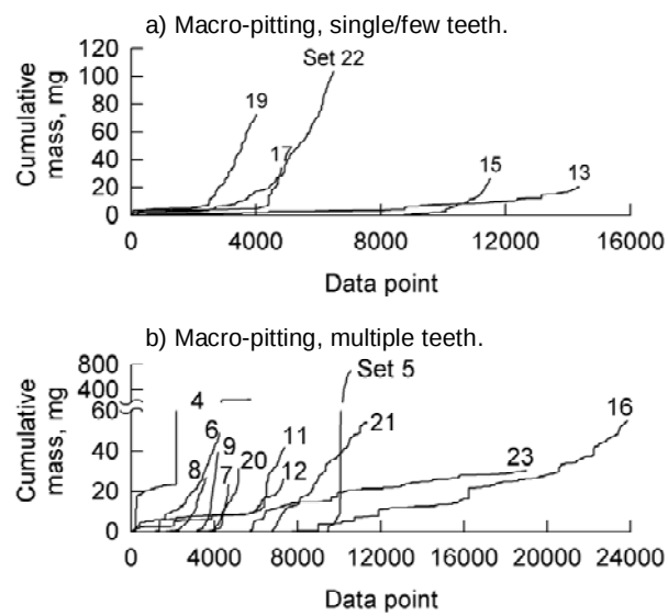
Figure 15. Oil-debris monitor results.
