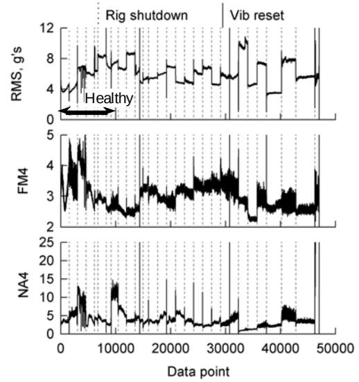
Figure B3. Set 3 vibration fault detection data.
