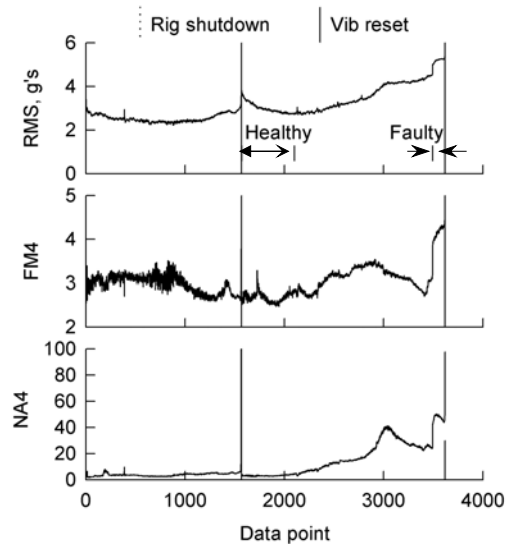
Figure B8. Set 8 vibration fault detection data.
