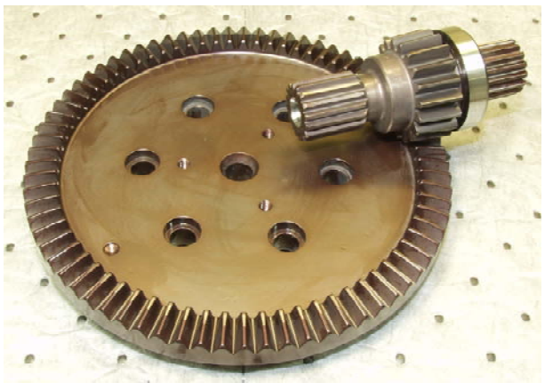
Figure 2. Test gears.
