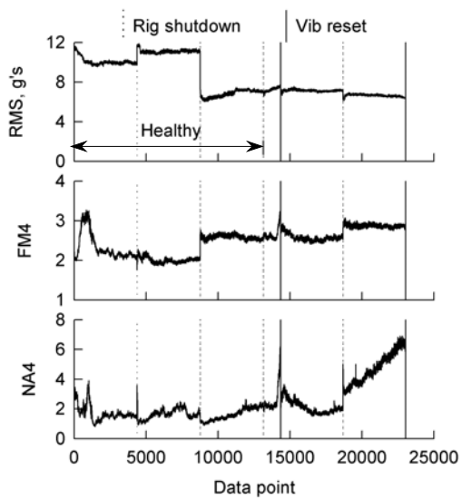
Figure B14. Set 14 vibration fault detection data.
