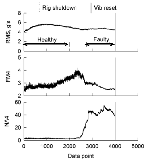
Figure B19. Set 19 vibration fault detection data.
