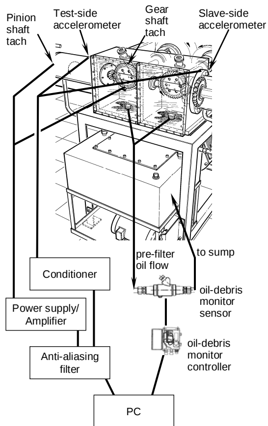
Figure 3. Gear fault detection instrumentation.
