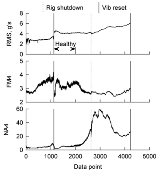
Figure B6. Set 6 vibration fault detection data.
