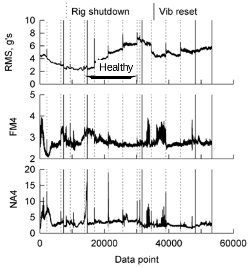
Figure B10. Set 10 vibration fault detection data.
