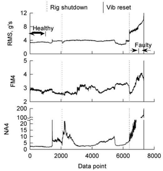
Figure B12. Set 12 vibration fault detection data.
