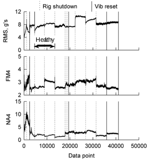
Figure B1. Set 1 vibration fault detection data.
