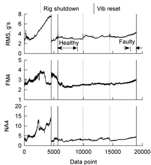
Figure B23. Set 23 vibration fault detection data.
