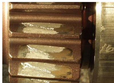
b) Multiple teeth macro-pitting failure.
