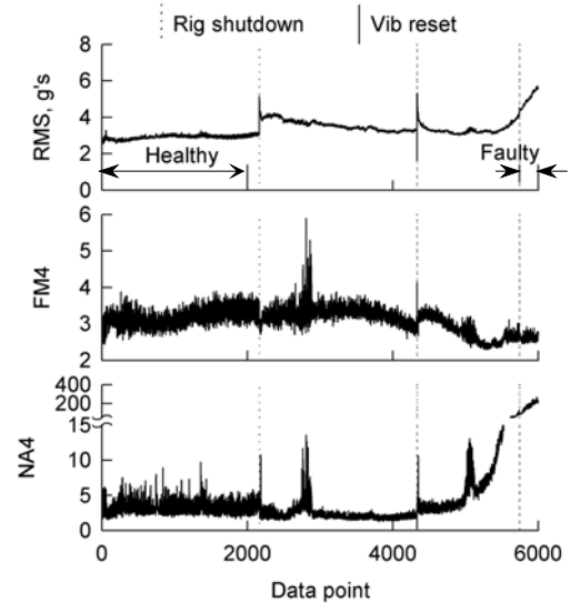
Figure B4. Set 4 vibration fault detection data.
