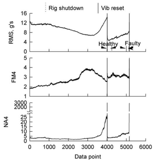
Figure B20. Set 20 vibration fault detection data.
