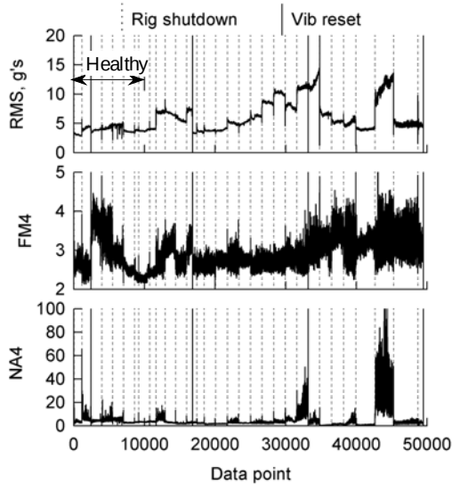
Figure B2. Set 2 vibration fault detection data.
