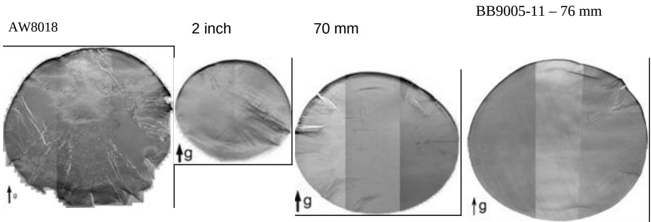
Grazing incident X-ray topographs of a typical SSM1 wafer, a 2-inch DCCS expansion wafer, a 70 mm DCCS expansion and a 76 mm DCCS expansion wafer.
