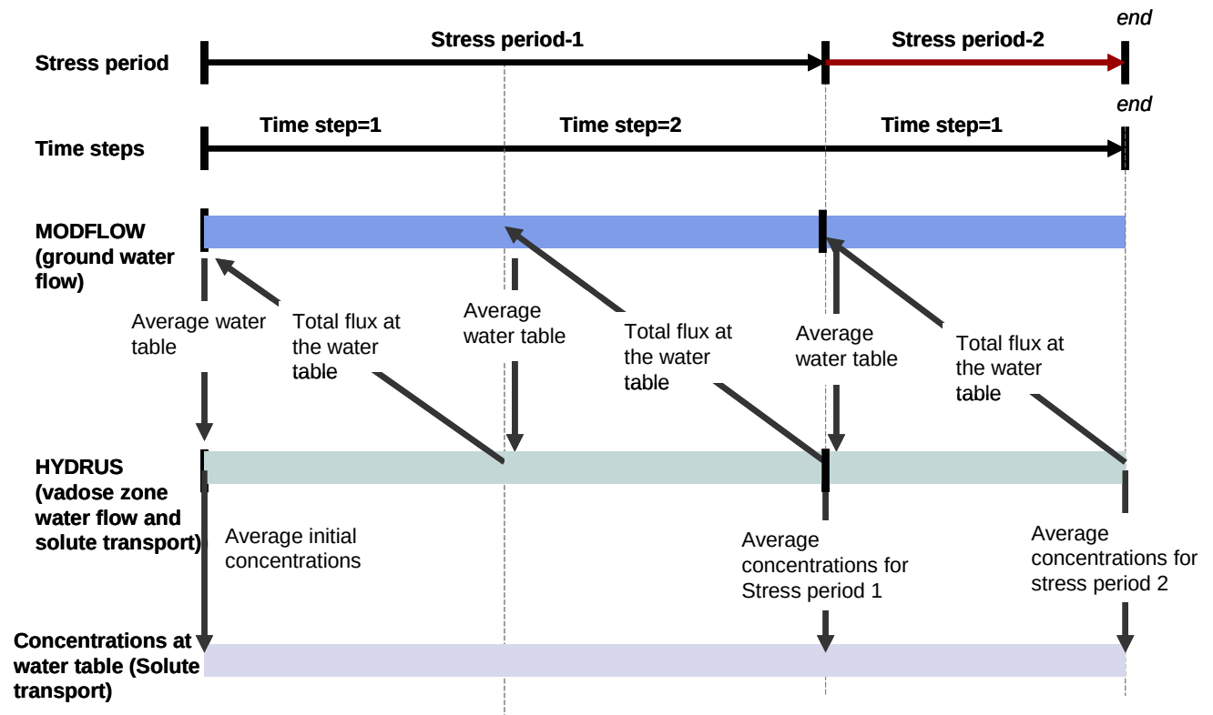
Figure 5. A schematic description of the coupling procedure for water flow and solute transport in HYDRUS-MODFLOW.
