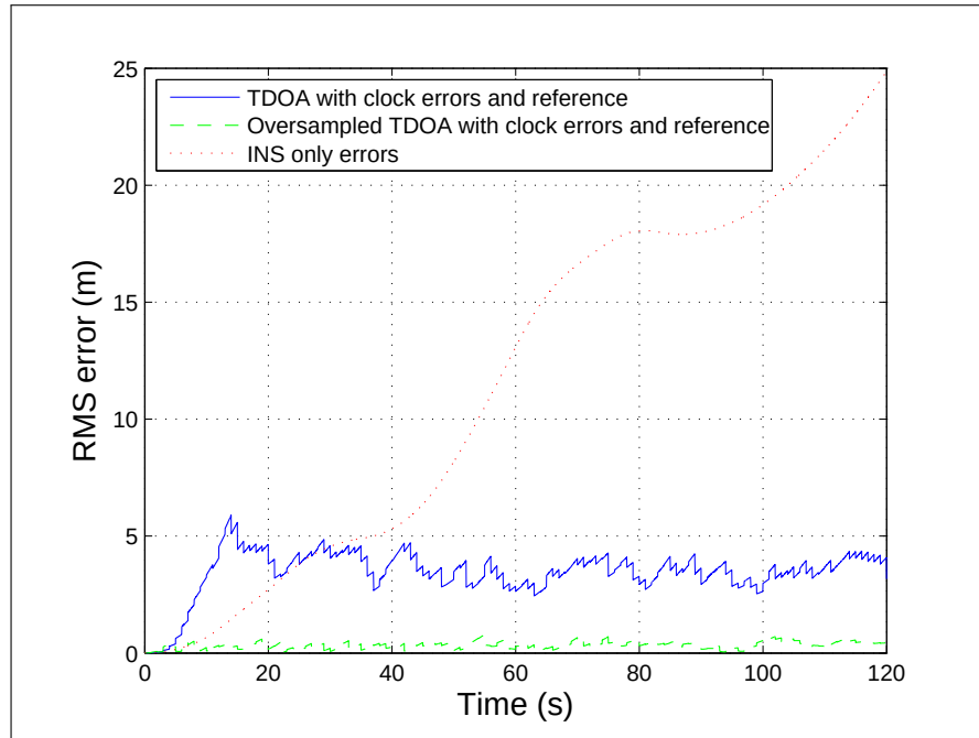
Figure 4.15: RMS errors over 10 runs versus time for both 20 MHz and 300 MHz sampling frequencies. Reference receiver has been added to correct clock errors.
