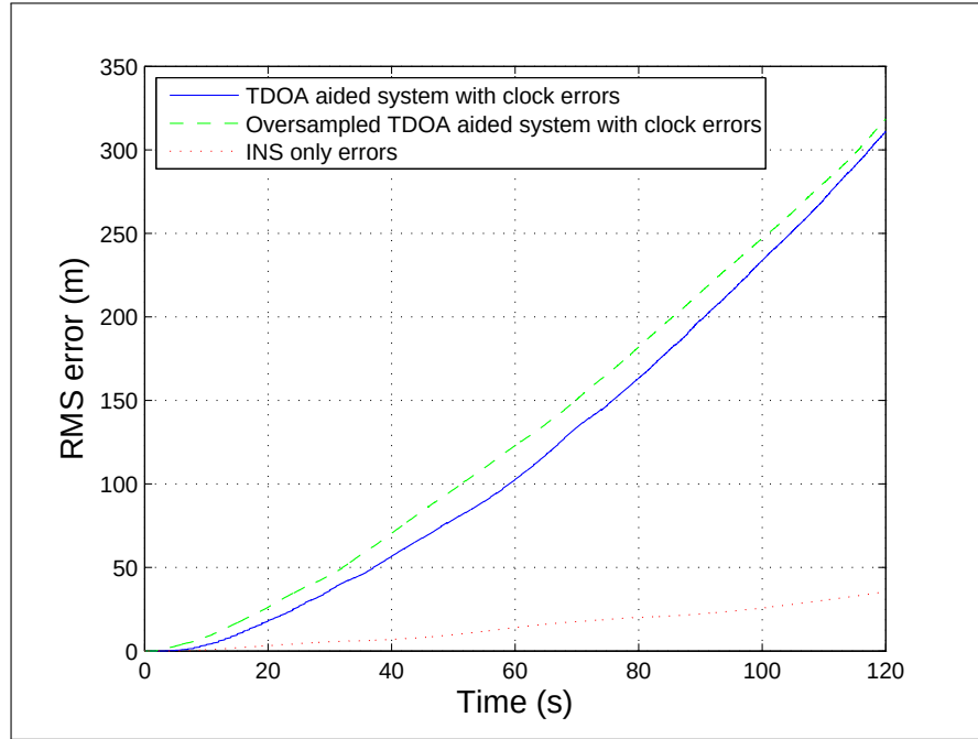
Figure 4.14: RMS errors over 10 runs versus time for both 20 MHz and 300 MHz sampling frequencies. Clock errors have been introduced and cause the error to grow over time.
