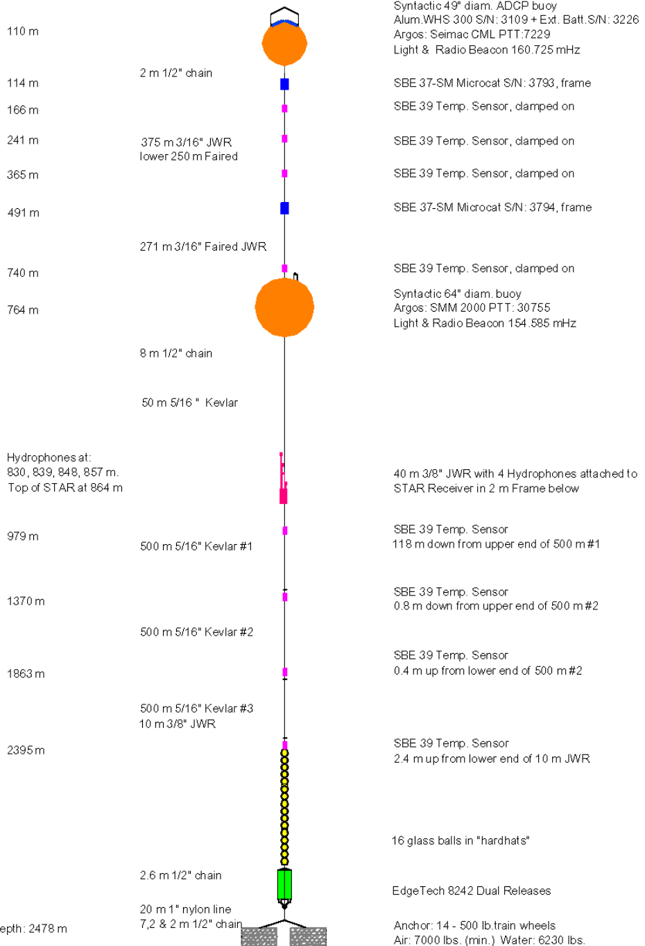
Figure 39. B1 mooring design, as deployed February 21, 2006.
