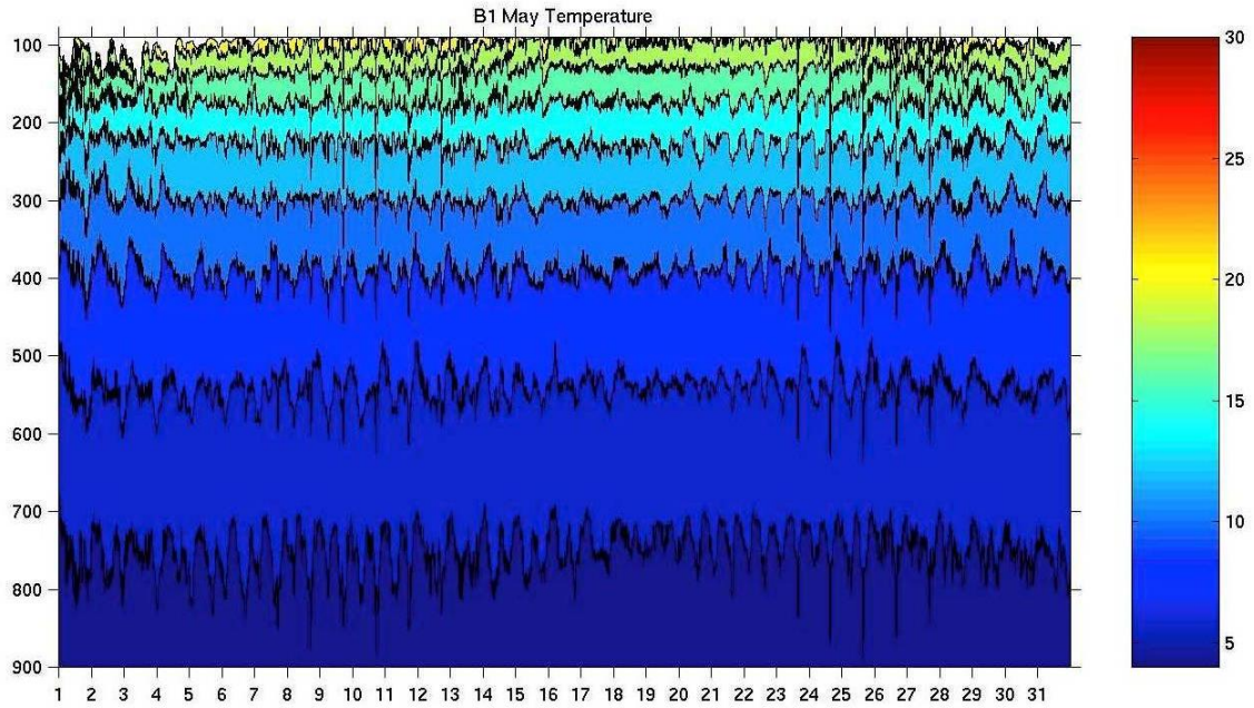
Figure 60. May 2005 temperatures (°C) at the B1 mooring, 100-900m.
