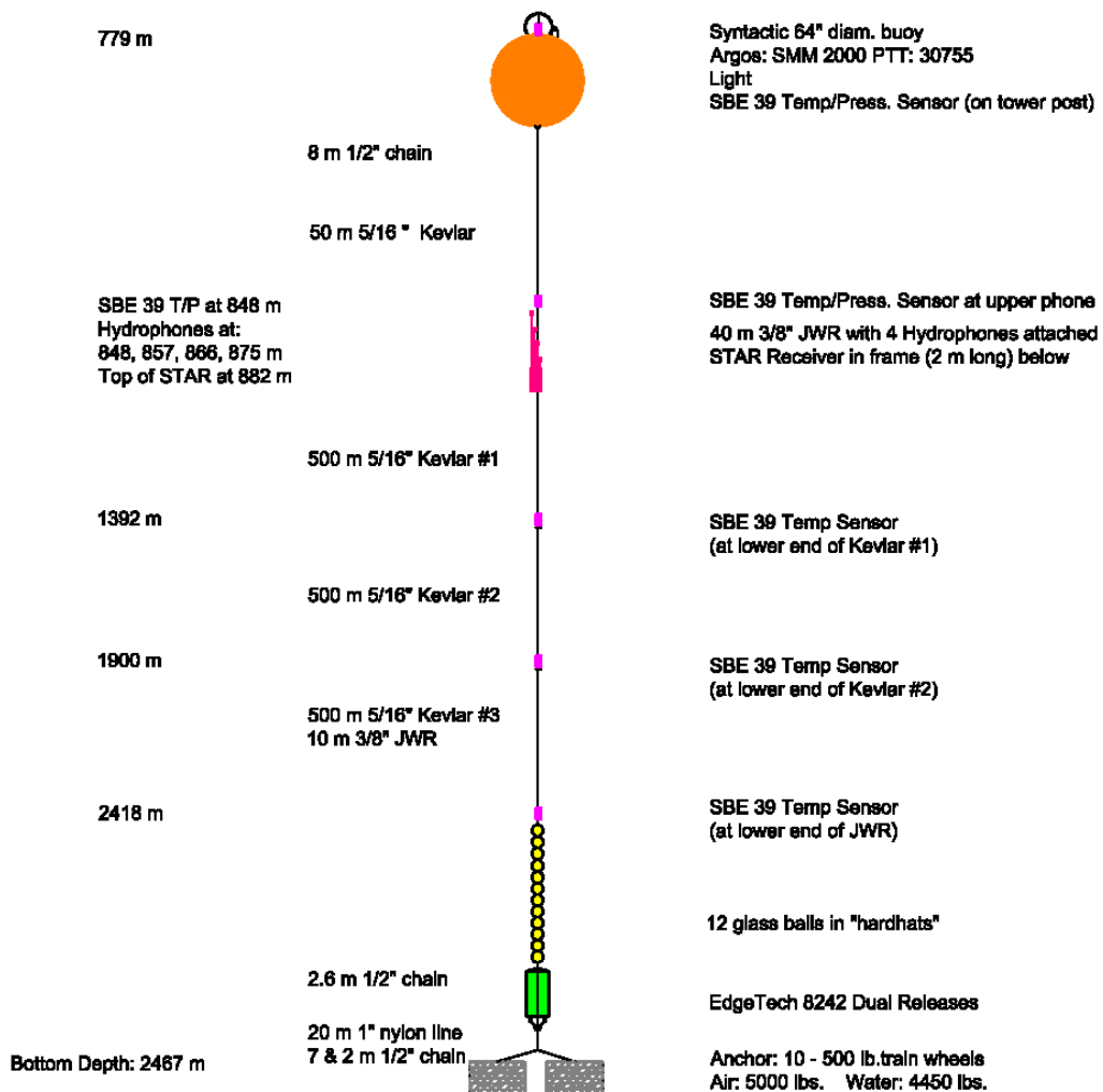
Figure 50. B1 mooring drawing, as deployed June 4, 2006.
