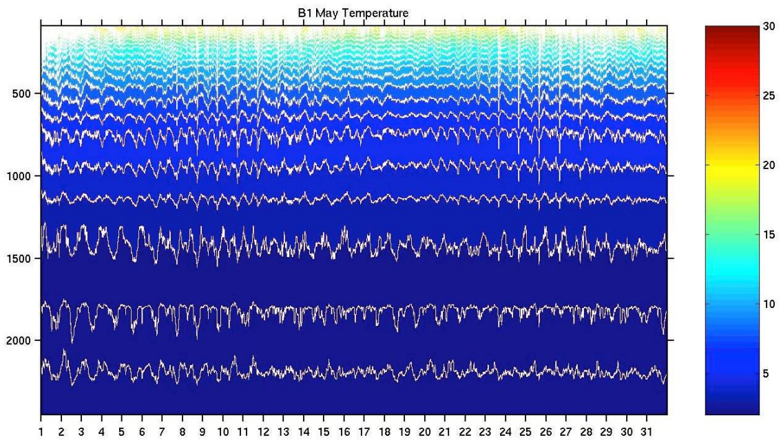
Figure 61. May 2005 temperatures (°C) at the B1 mooring.
