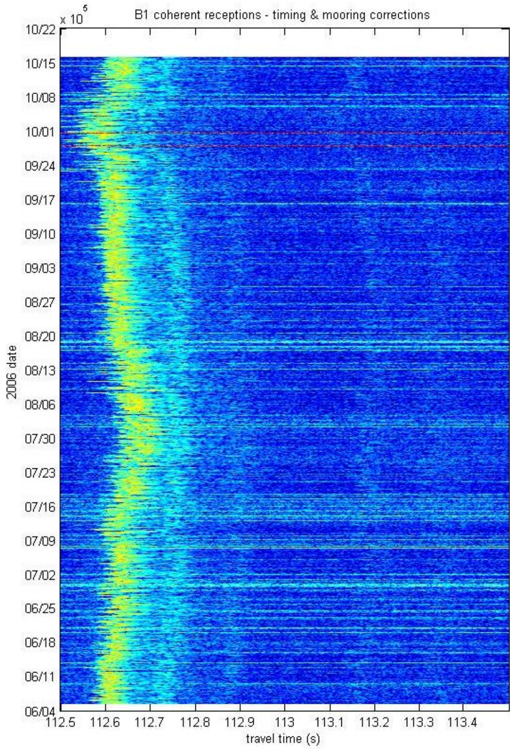
Figure 49. Acoustic arrival structures over the June-October 2006 deployment.
