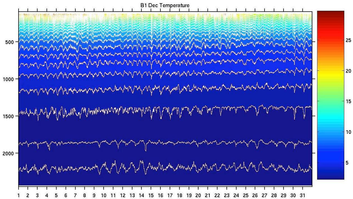
Figure 79. December 2005 temperatures (°C) at the B1 mooring.
