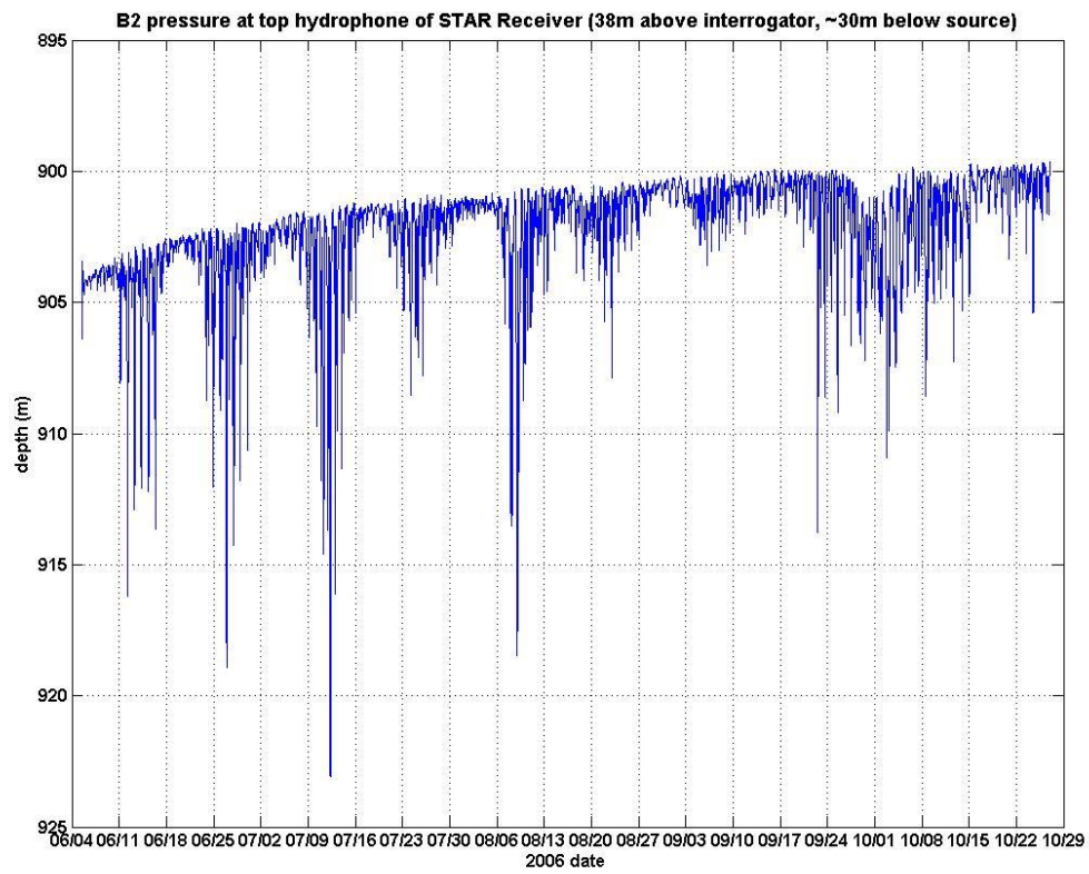
Figure 51. B2 Pressure sensor at top STAR hydrophone.
