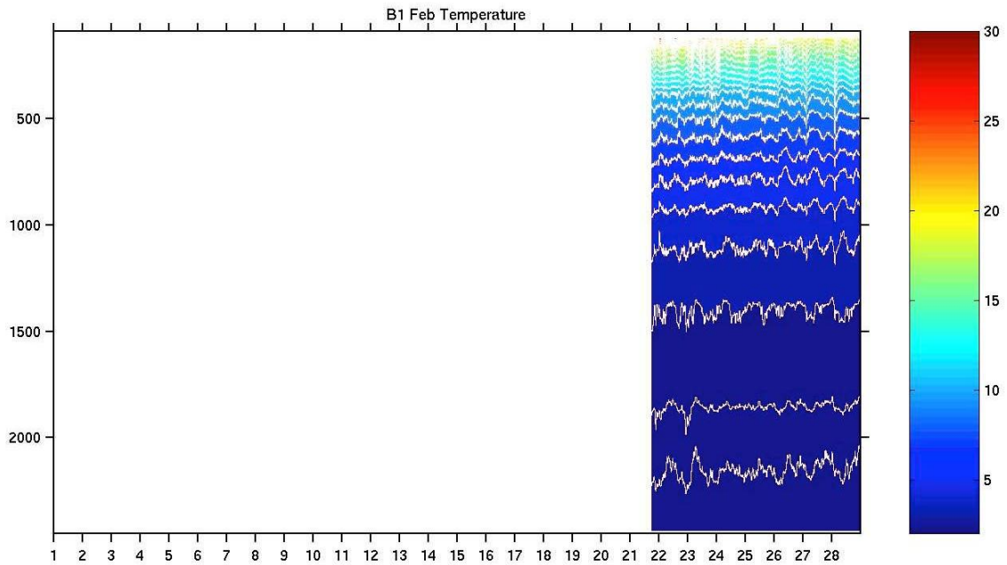
Figure 85. February 2006 temperatures ( ^{\circ}\text{C} ) at the B1 mooring (cont).
