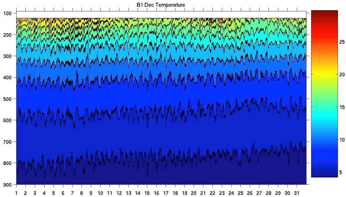
Figure 78. December 2005 temperatures (°C) at the B1 mooring, 100-900m.
