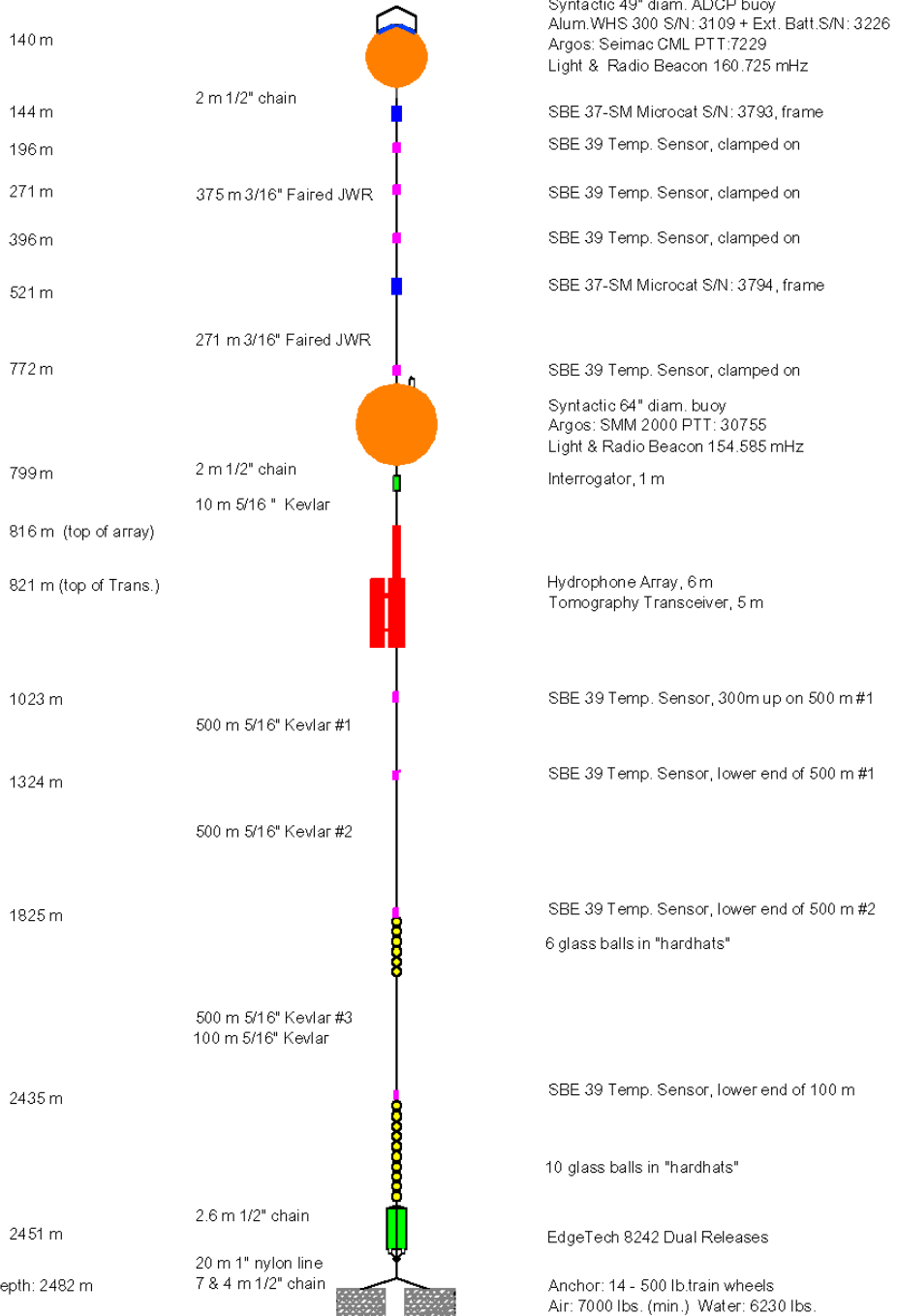
Figure 30. B1 mooring design "as deployed" July 27, 2005.
