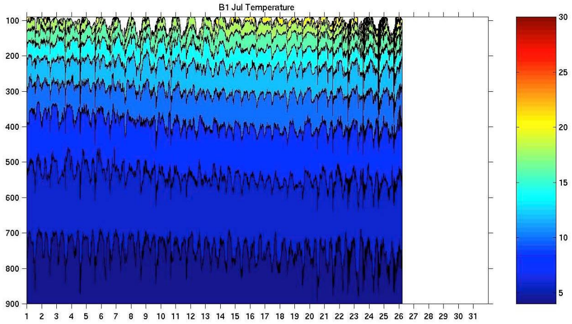
Figure 64. July 2005 temperatures (°C) at the B1 mooring, 100-900m.
