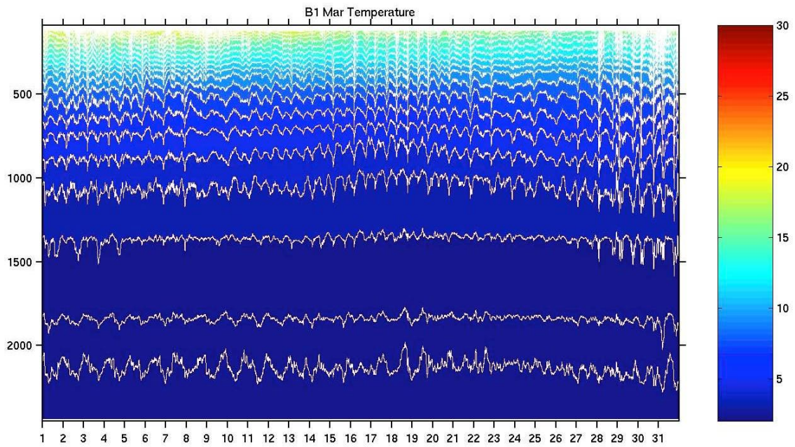
Figure 87. March 2006 temperatures (°C) at the B1 mooring.
