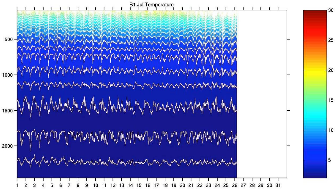
Figure 65. July 2005 temperatures (°C) at the B1 mooring.
