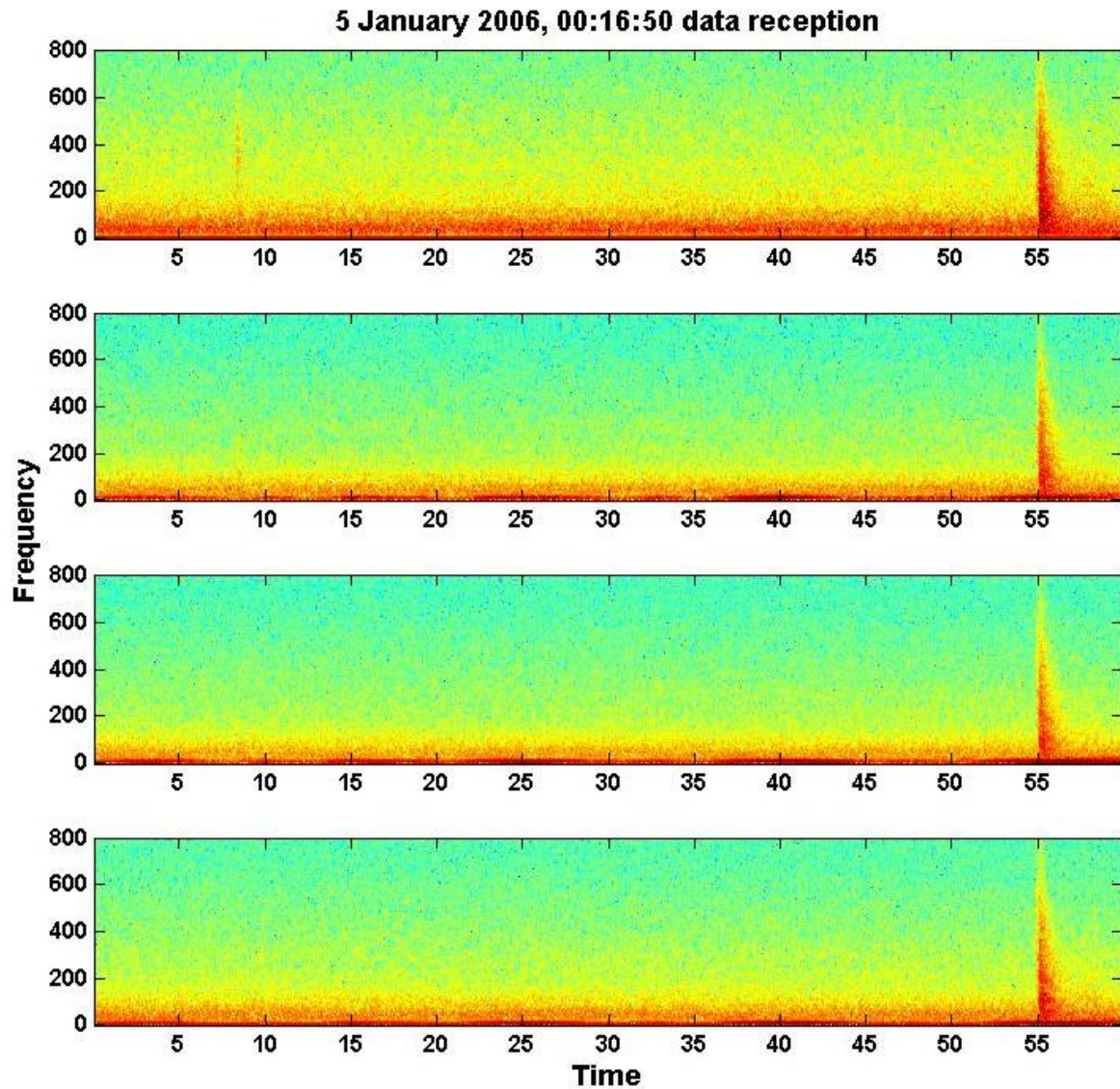
Figure 40. Receiver data spectrograms from the B1 STAR hydrophones showing the broadband point sources (~55 seconds into the files) typical of the local Chinese fishing activity.
