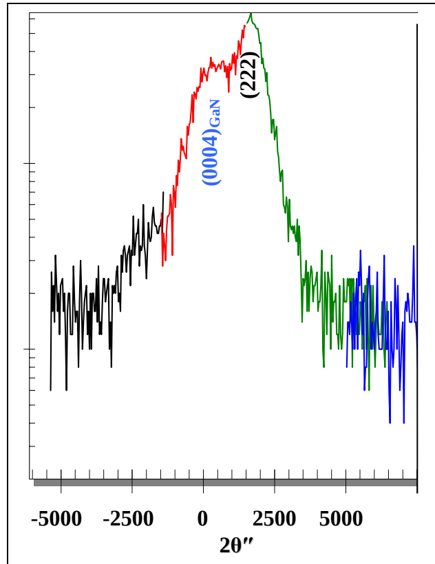
Figure 13b. Rocking curve for the (0004) GaN and (222) peaks.
