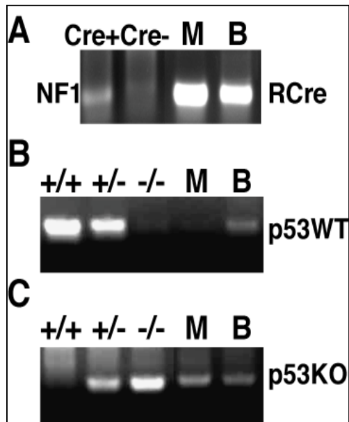
Figure 10. Molecular analysis of benign and malignant peripheral nerve sheath tumors. Benign and malignant portions of a tumor were isolated from LCM. (A) Both benign and malignant tumors underwent loss of Nf1 . Rcre represents the recombined flox allele. (B) Malignant, but not benign tumors, underwent loss of the wild type p53 allele. (C) Both malignant and benign tumors still retained the knockout p53 allele. M, malignant tumor; B, benign tumor.
