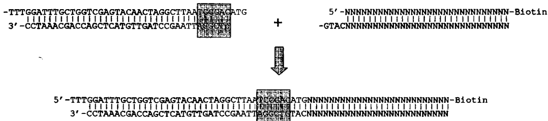
Fig. 16.4. Cassette A, Mme I restriction site and ligation of cassette A.
