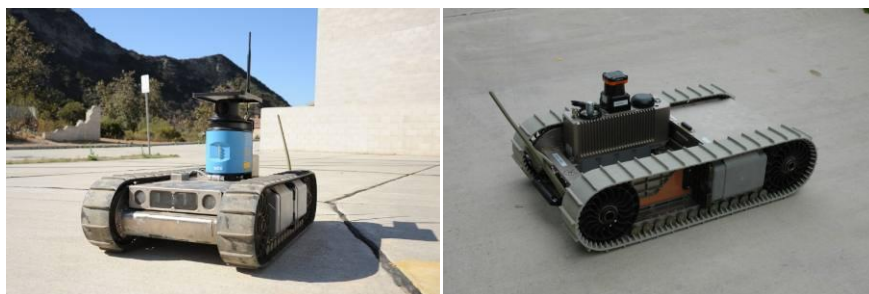
Figure 2. First generation of iRobot's Navigator Payload used for UrbEE testing in FY08 (left); 2 nd generation planned for use in FY09 testing (right).
