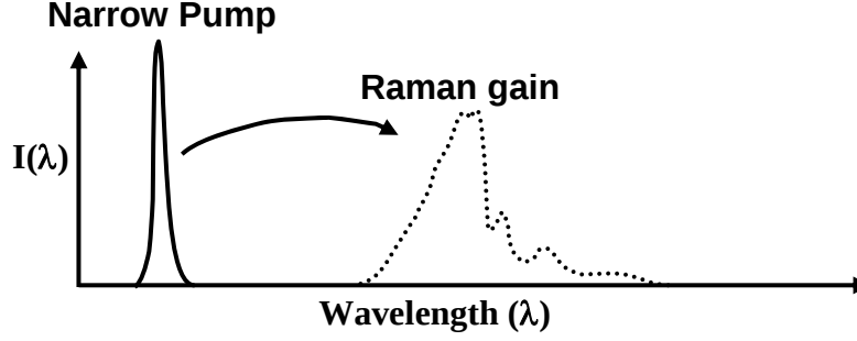
Figure 1 Illustration showing the silica Raman gain produced by a bright incident laser.
