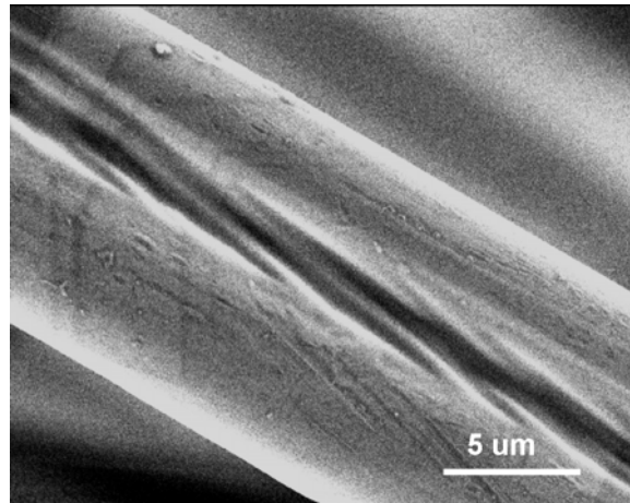
Figure 4.16: SEM micrographs of PBO AS fiber surfaces after compaction in scCO 2 and silicon oil.
