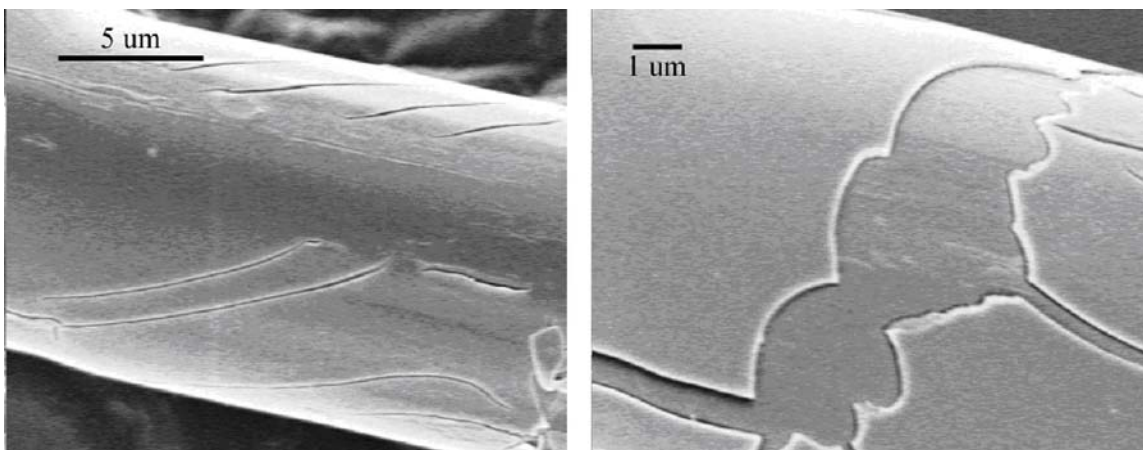
Figure 4.13: SEM of \text{TiO}_2 coating showing a thin film with thickness on the order of \sim 100 's of nanometers.
