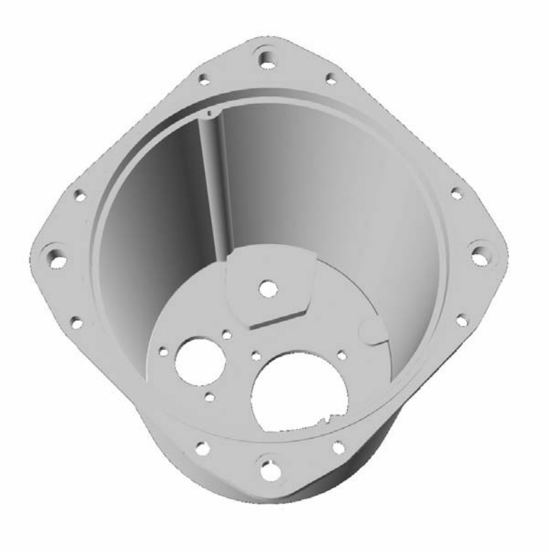
Figure 4.3 3D model of the airspeed indicator case, developed at the University of Utah.
