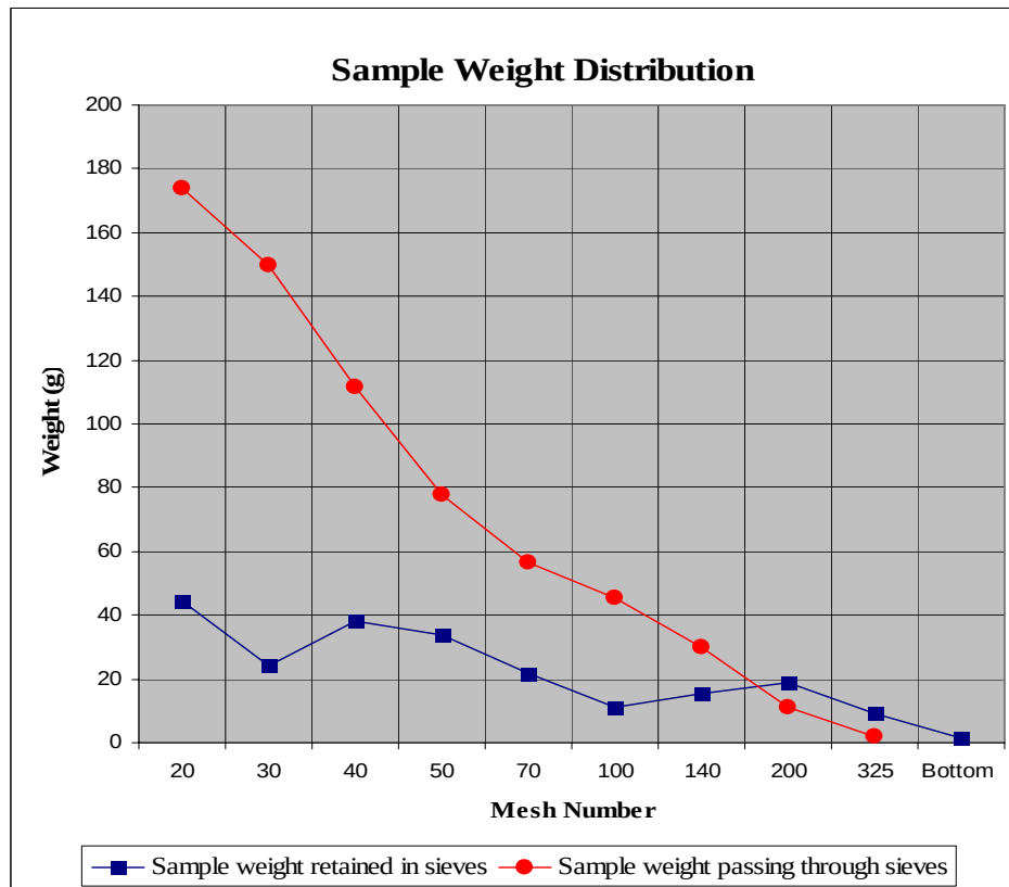
Figure B-3. Graphical Depiction of Sand Particle Distribution by Weight
