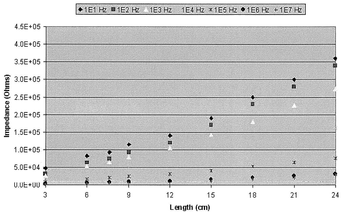
Figure A3: Plant 2142: Impedance versus Length for Various Frequencies
