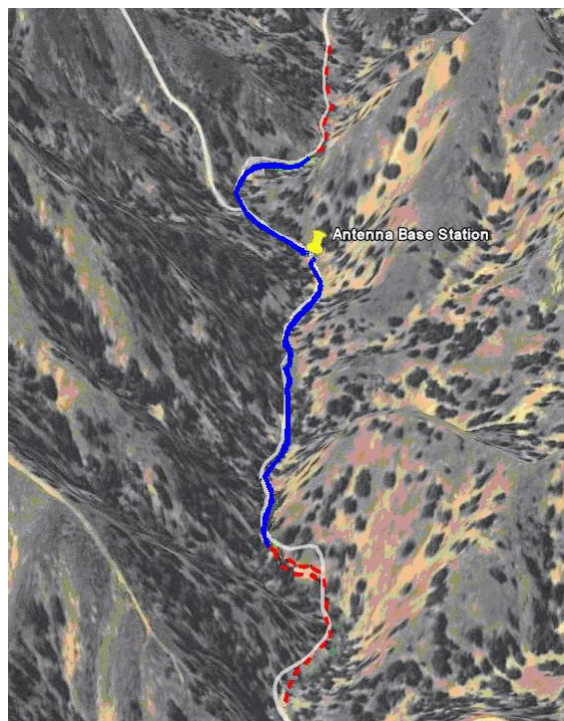
Figure 12. Example display of radio field test results showing active (blue solid) and broken (red dashed) communication links between a static base station and mobile platform
