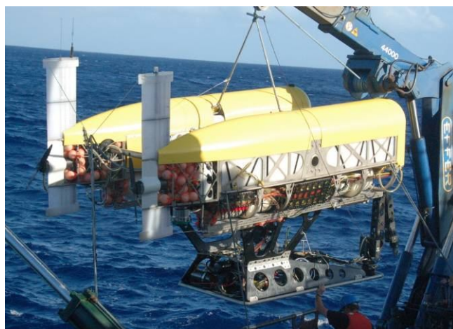
Figure 16. Nereus in the ROV Configuration.
