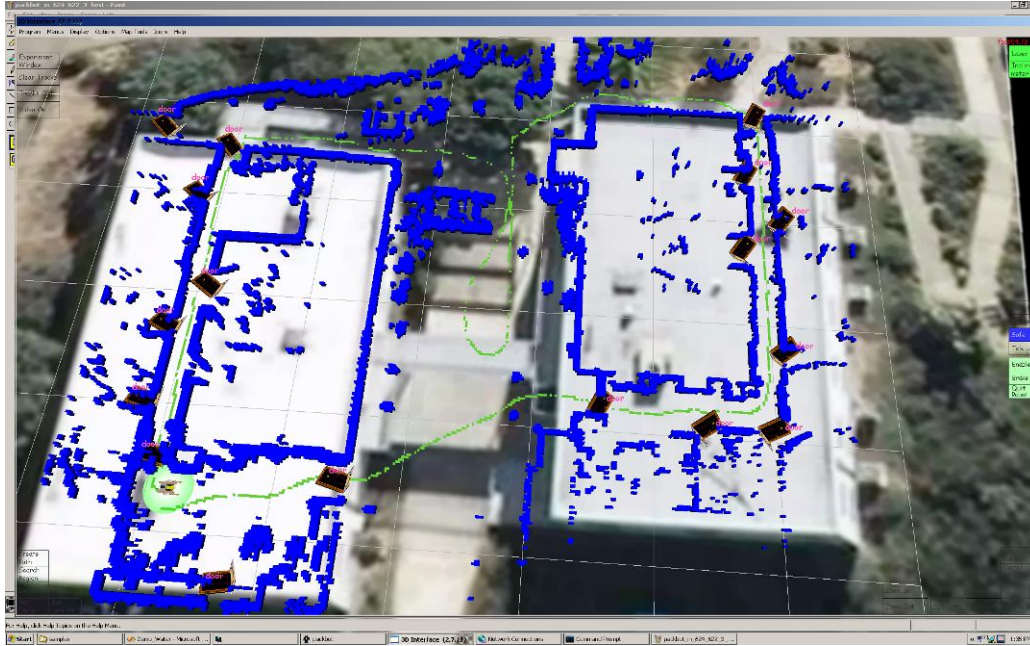
Figure 2. A SLAM map registered with aerial imagery in real time.
