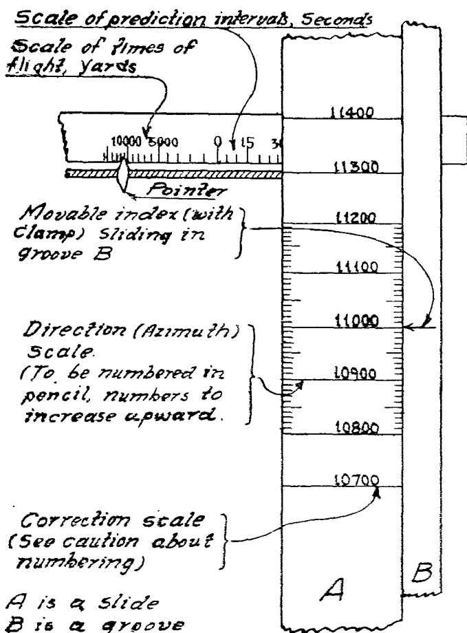
FIG. 1. VERTICAL T-SQUARE OF AZIMUTH PREDICTION BOARD
