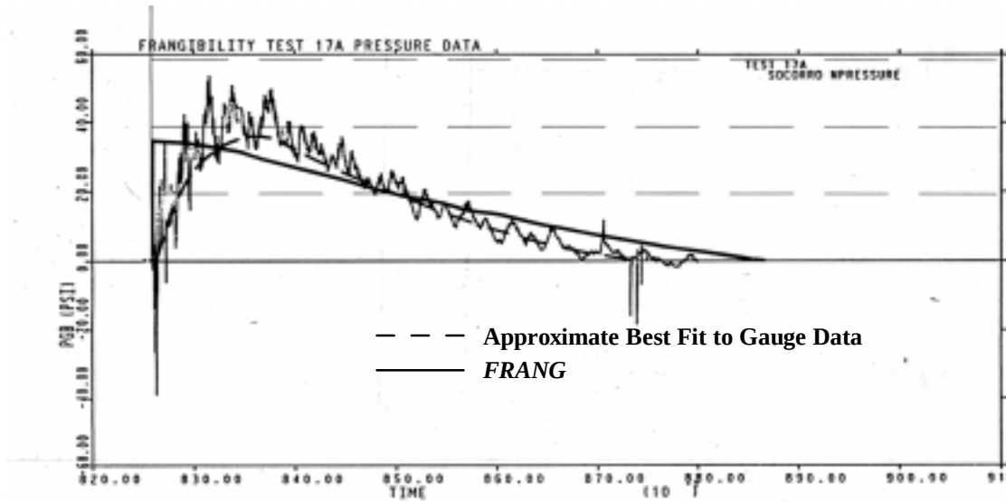
Figure B-2. Test 17: Gas Pressure Gauge Data vs. FRANG Results W/V = 0.0044 , A/V^{2/3} = 0.20 , w/W^{1/3} = 12.3
