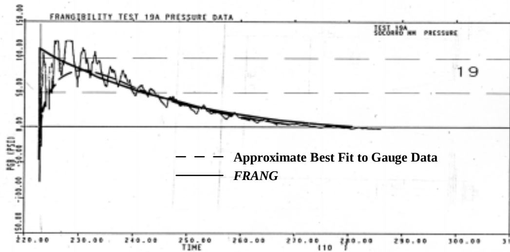
Figure B-3. Test 19: Gas Pressure Gauge Data vs. FRANG Results W/V = 0.0178 , A/V^{2/3} = 0.20 , w/W^{1/3} = 0
