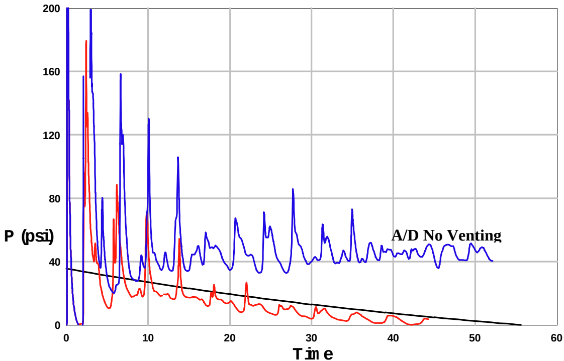
Figure 3. P_g(t) : AUTODYNE ( A/D ) and FRANG ( W = 2 \text{ lb.} , W/V = 0.0044 , A/V^{2/3} = 0.20 , Test #9)
