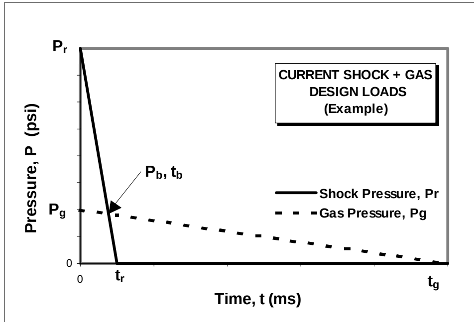
Figure 2. Current Design Internal Pressure Loads (Ref. (6))
