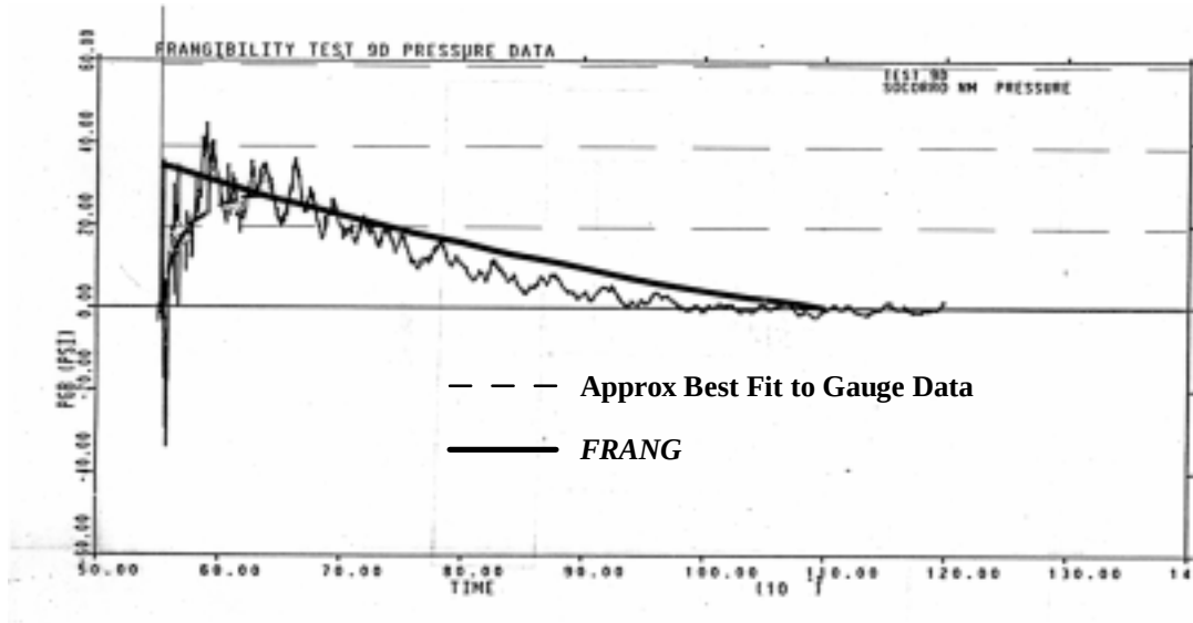
Figure B-1. Test 9: Gas Pressure Gauge Data vs. FRANG Results W/V = 0.0044 , A/V^{2/3} = 0.20 , w/W^{1/3} = 0
