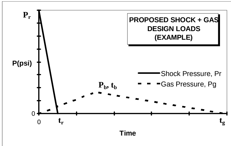
Figure 4. Proposed Design Internal Pressure Loads
