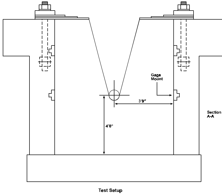
Figure 1. Test Setup
