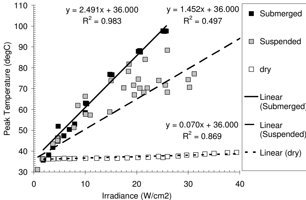
Figure 5. Peak temperature during laser exposure is obtained from thermal images and plotted against irradiance. Three membrane conditions were examined: wetted with HBSS with full contact from below (submerged), wetted then suspended in air (suspended), and dry (as received from manufacturer). Trendline y-intercept values were forced to 36°C (average temperature of the thermal box) for ease of comparison.
