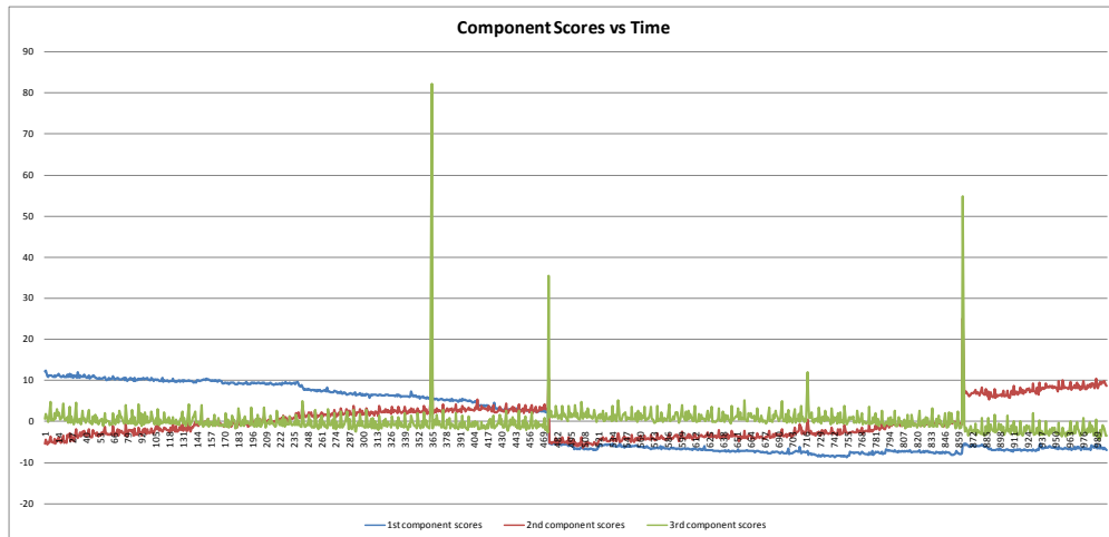
Figure 18 – Nov 7 Run3 First Three PCA Scores vs. Time
