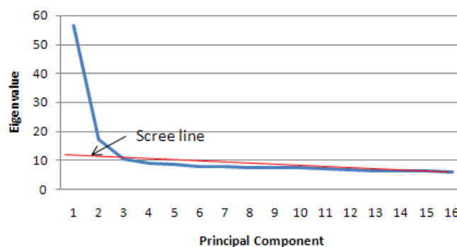
Figure 5 – Cattell's Scree Test
