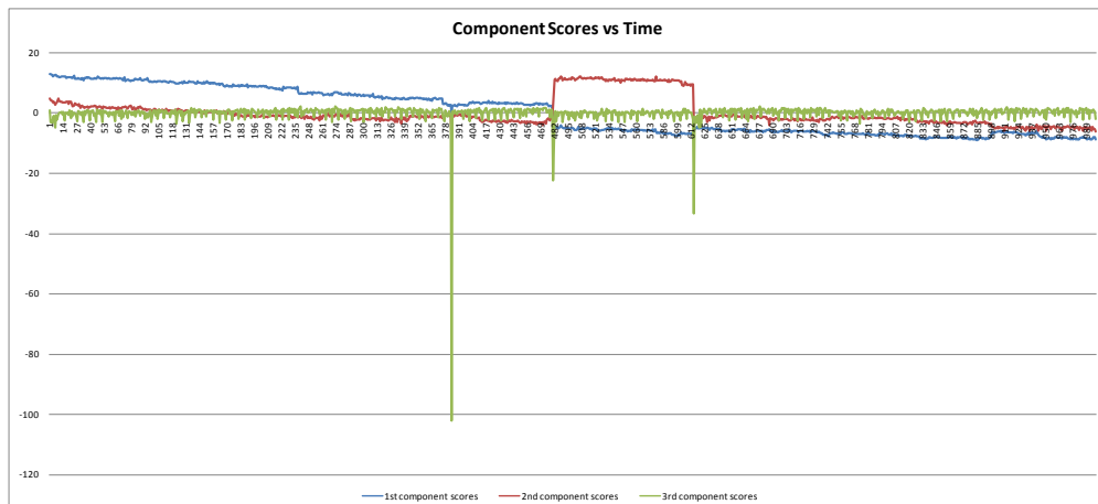
Figure 17 – Nov 7 Run2 First Three PCA Scores vs. Time
