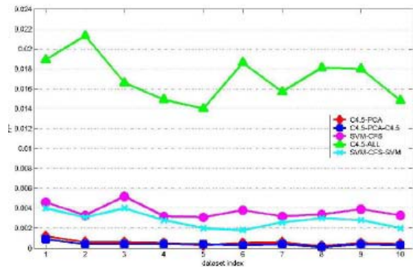
Figure 4. False positive rates vs. dataset index
