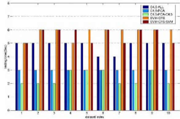
Figure 2. System testing time vs. dataset index
