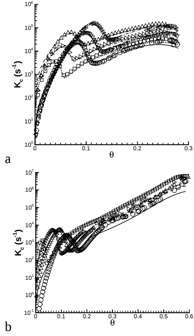
Fig. 4: K_c versus \theta for a variety of conditions. Symbols \square , \triangleright , \Delta , \bigcirc , \nabla , \triangleleft represent selected data from the LLNL runs; lines \bullet\bullet\bullet , -\bullet-\bullet- , --- , --- , --- , -\bullet\bullet-\bullet\bullet- represent the corresponding fits. Units: pressures in bar, temperatures in degrees K. (a) \phi = 4 , ( \bullet\bullet\bullet p_0 = 10 , T_s = 825 ; --- p_0 = 10 , T_s = 715 , -\bullet-\bullet- p_0 = 20 , T_s = 825 ; --- p_0 = 20 , T_s = 715 ; --- p_0 = 40 , T_s = 825 ; -\bullet\bullet-\bullet\bullet- p_0 = 40 , T_s = 715 ). (b) p_0 = 10 and \phi = 1 ( \bullet\bullet\bullet T_s = 825 ; --- T_s = 715 , -\bullet-\bullet- T_s = 655 ; --- T_s = 560 ).
