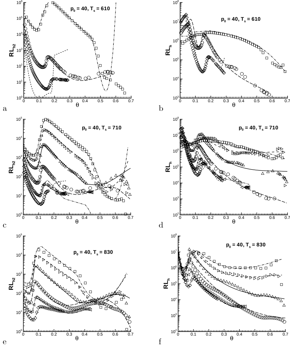
Figure 3. RL versus \theta for p_0 = 40 bar at different T_s values. Symbols \square, \triangleright, \triangle, \bigcirc, \triangleleft, \diamond represent selected results using the LLNL database; lines represent the corresponding fits. Temperatures units are in degrees K. The legend is: \square , -\bullet-\bullet- \phi = 1/4 ; \triangleright , - - - \phi = 1/3 ; \triangle , --- \phi = 1/2 ; \bigcirc , --- \phi = 1 ; \triangleleft , -\bullet-\bullet- \phi = 2 ; \diamond , \bullet\bullet\bullet \phi = 4 . (a,c,e) for H_2 and (b,d,f) for H .
