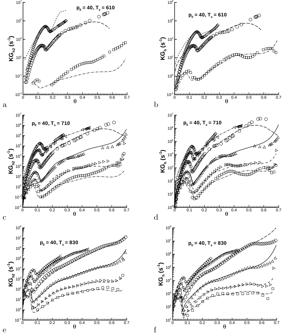
Figure 2. KG versus \theta for p_0 = 40 bar at different T_s values. Symbols \square , \triangleright , \Delta , \bigcirc , \triangleleft , \diamond represent selected results using the LLNL database; lines represent the corresponding fits. Temperatures units are in degrees K. The legend is: \square , — \bullet — \bullet — \phi = 1/4 ; \triangleright , - - - \phi = 1/3 ; \Delta , — \phi = 1/2 ; \bigcirc , - - - \phi = 1 ; \triangleleft , - \bullet — \bullet — \phi = 2 ; \diamond , \bullet — \bullet — \phi = 4 . (a,c,e) for \text{H}_2 and (b,d,f) for \text{H} .
