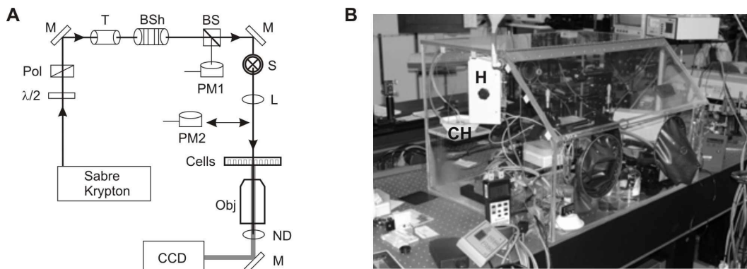
Fig. 1 Laser delivery for in vitro damage threshold experiments. Panel A: M, mirror; \lambda/2 , half-wave plate; Pol, polarizing beam splitter; T, optical telescope; BSh, beam shaper; S, shutter; L, lens; PM, power meter; ND, neutral density filter; CCD, charge-coupled device camera; Obj, microscope objective. Panel B: Photograph of environmentally controlled laser exposure enclosure. H, high capacity air-driven heater; CH, cartridge heater placed in a container of water for generation of humidity.
