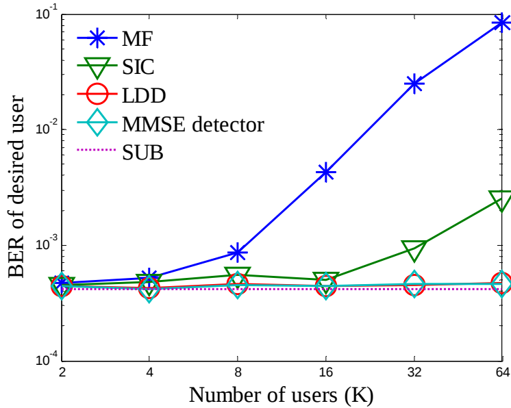
Fig. 9 BER vs. number of users in the adaptive system with imperfect power control for M=12 , N=8 , PG=64 , \eta=0.95 , and \Delta f\sigma_d=0.1024 . The SNR is 10dB for desired user and 20dB for other users.
