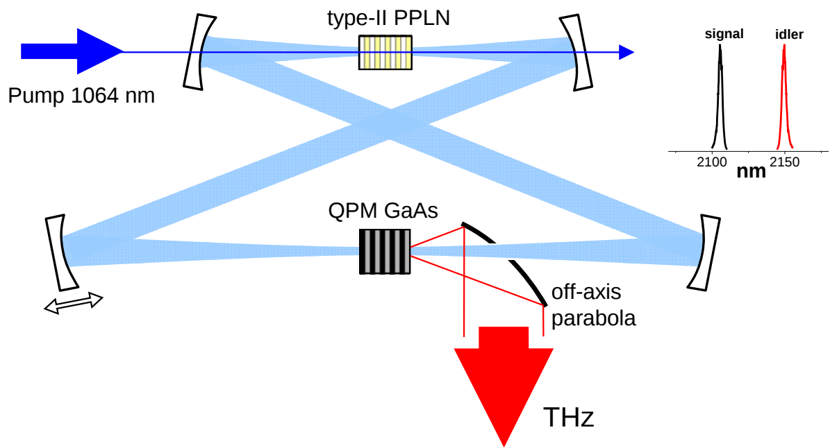
Figure 17. Conceptual schematic of the setup for resonantly-enhanced THz-wave generation in a ring OPO cavity.
