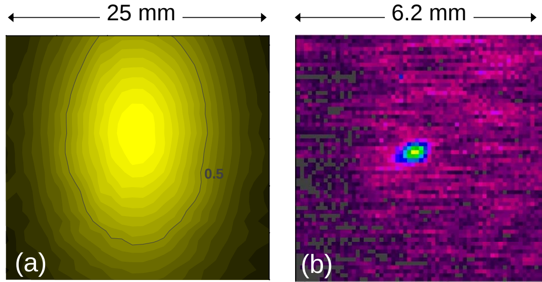
Figure 13 (a) Collimated THz-beam intensity profile reconstructed from scanning knife-edge measurements. (b) Focused ( f=50 mm lens) THz-beam intensity profile measured by a room-temperature pyroelectric camera (1 pixel= 100 \times 100 \mu\text{m} ).
