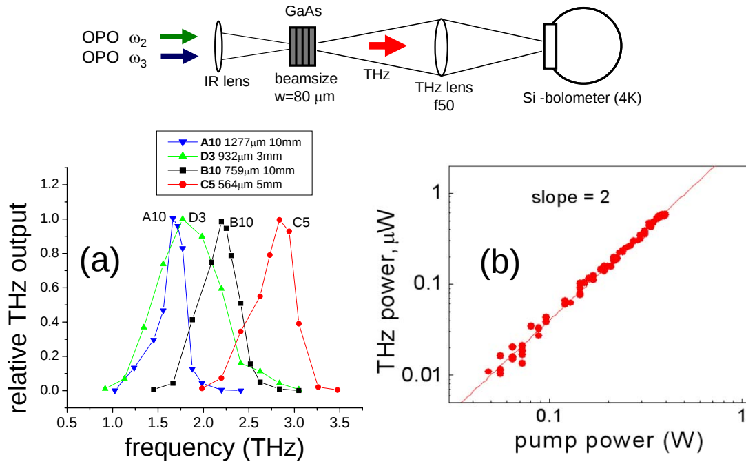
Figure 9 (a) THz output vs. frequency in the DFG experiment outside the OPO cavity, for 4 OP-GaAs samples with different lengths (3-10 mm) and QPM periods (564-1277 \mu\text{m} ). (b) THz average output power versus incoming average pump power for a 5-mm-long uncoated OP-GaAs sample (QPM period 704 \mu\text{m} , center frequency 2.2 THz). Straight line is the best fit.
