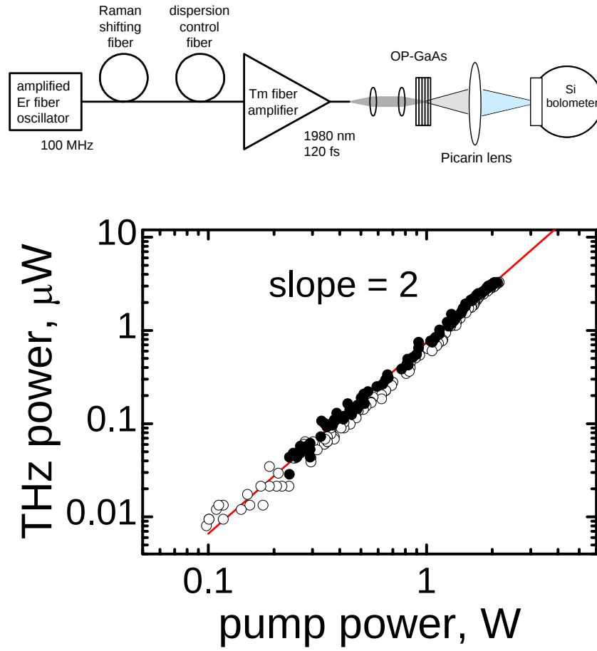
Figure 5 Schematic of the OR THz experiment with a 2- \mu\text{m} fiber laser. THz average power vs. laser pump power for the OP-GaAs samples A3 (filled circles) and B3 (open circles). Straight line is the best fit for the A3 data.
