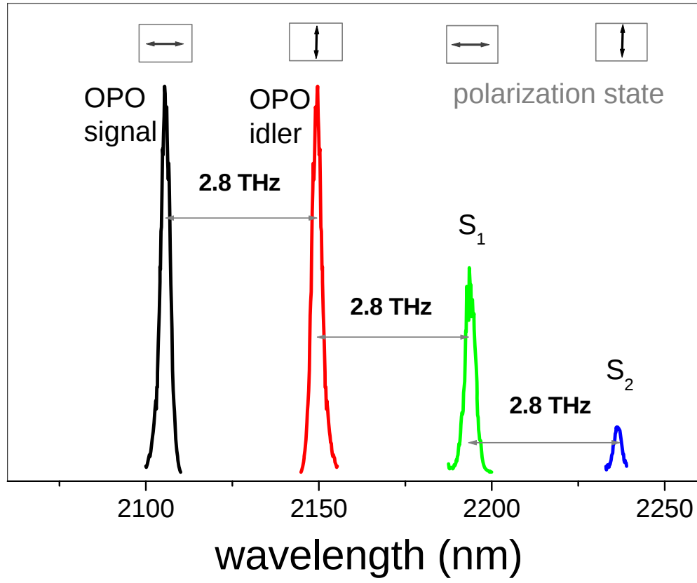
Figure 14 Spectrum of the optical radiation (not to scale) in the intracavity SRO DFG experiment with the 6-mm DB-GaAs sample (center frequency 2.8 THz). In addition to the signal and the idler peaks, one can see two additional red-shifted peaks, corresponding to the 1-st and the 2-nd cascaded satellites S_1 and S_2 . Polarizations states of the peaks are shown on the top.
