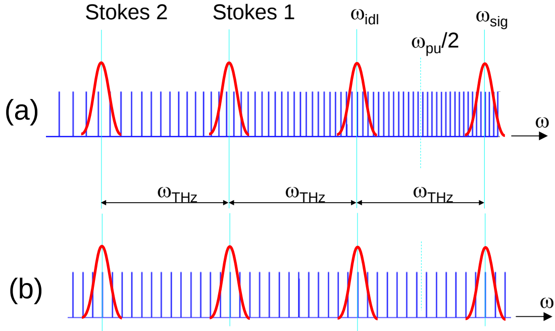
Figure 15 (a) Case of non-zero group velocity dispersion (GVD). The OPO resonator modes are not equidistant and it is impossible to achieve resonant condition for the 1-st and higher Stokes frequencies. (b) When GVD is eliminated, simultaneous resonance can be achieved in the whole frequency range.
