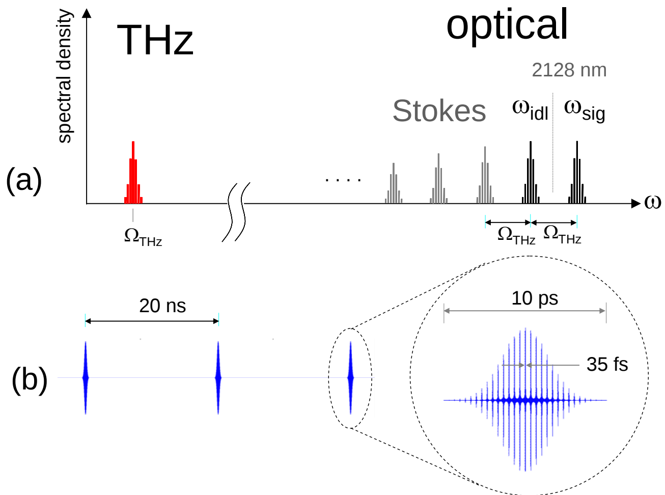
Figure 16. (a) Frequency modes for the OPO signal, idler, Stokes frequencies, as well as for THz wave. (b) Time domain picture. When the modes of the signal, idler and several ( \sim 8 ) Stokes frequencies are resonant and phase-locked, the optical pulse consists of extremely short ( \sim 35 fs) bursts of radiation.
