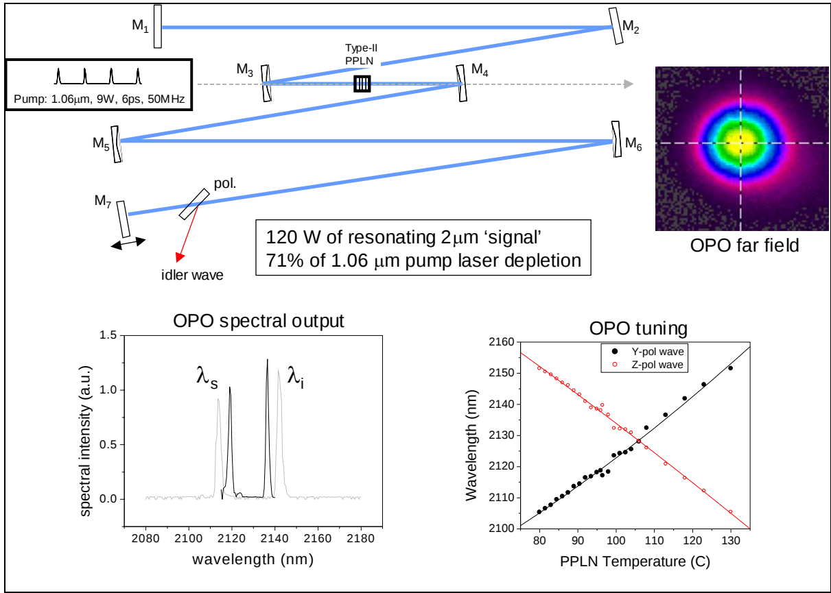
Figure 8 Near –degenerate type-II PPLN OPO, synchronously pumped by ps pulses at 1.06 \mu m. Insets: ‘signal’ wave far field intensity distribution, spectral output of the OPO at two different PPLN temperatures, and OPO tuning curve with respect to PPLN temperature.
