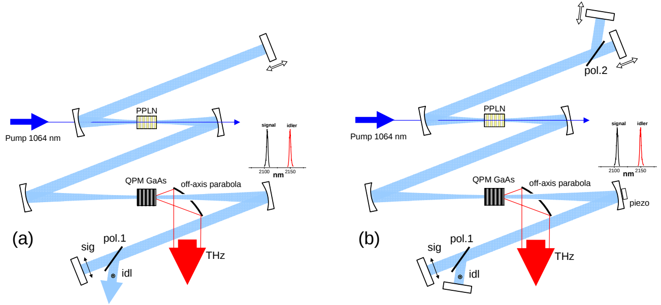
Figure 11 Setup for THz generation using GaAs inside the cavity of a near –degenerate synchronously-pumped PPLN OPO. (a) Singly-resonant OPO (SRO), (b) doubly-resonant OPO (DRO). Off-axis parabolic mirror with a hole in the center was used to extract the THz output.
