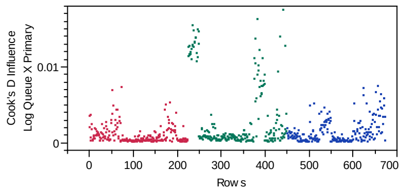
Cooks Distance Plot
