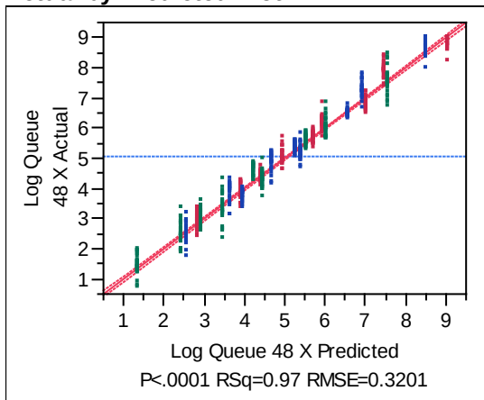
Summary of Fit
