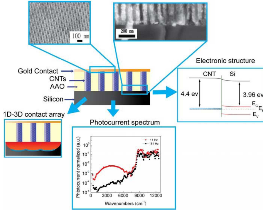
Fig.1 Some of the aspects of the carbon nanotube-Si heterojunction studied in this phase of development include: the temperature dependence of the CNT-Si heterodimensional heterojunction contacts, the temporal characteristics of the photocurrent generation mechanism, the reverse rectification behavior of the CNT-Si heterojunction at small currents, and the intensity dependence of the photoresponse
