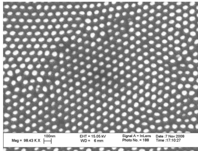
Fig. 12 Ordered gold nanoparticles on n-type silicon substrate formed by evaporating gold through an AAO mask.
