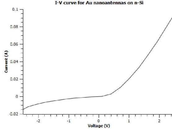
Fig. 13 I-V curve for the nanoantenna array sample with height of 800nm, diameter of 40nm and inter-antenna spacing of approximately 100nm.
