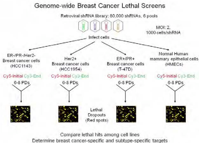
Figure 9. Breast cancer lethal screen design. A genome-wide lethality screen was performed in three breast cancer cell lines and one normal human mammary epithelial cell line for shRNAs against genes whose knockdown decreases viability of breast cancer but not normal cells. Such genes are novel cancer drug targets.
