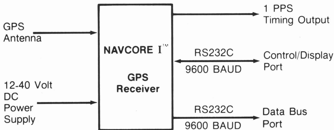
Figure 4. NAVCORE Block Diagram.
