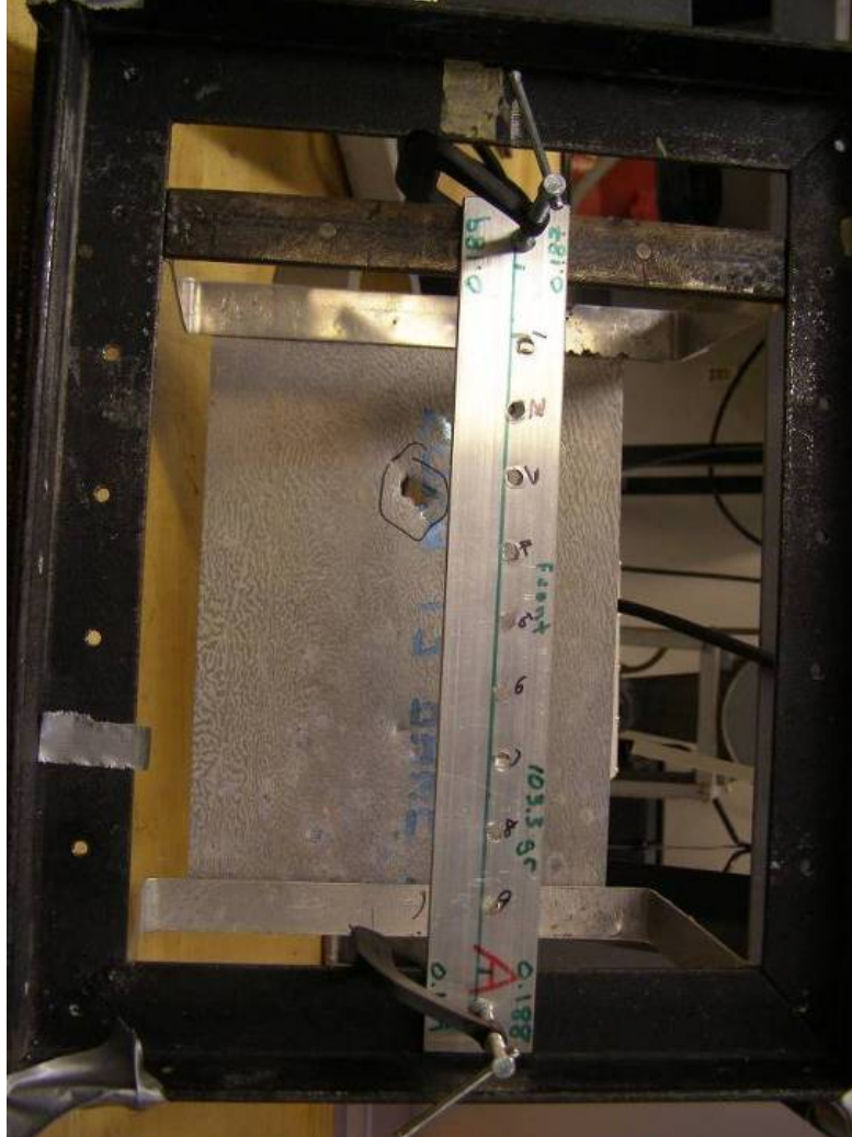
Figure A-2. A sample in the test rig with a 228- × 152.4- × 0.508-mm 2024Al witness plate placed 152 mm behind and parallel to sample. The distance between the clamps was 254 mm.
