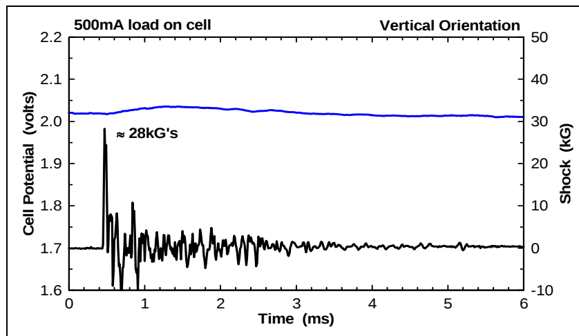
Figure 8. DLCR2 cell no. 3, shock test no. 2.
