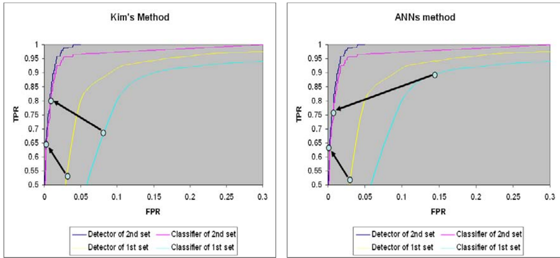
Figure 55: The Movement of the optimal points for Each Techniques (Label Accuracy for Enemy)
