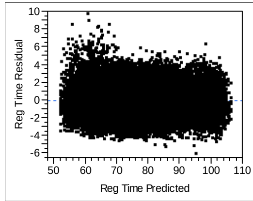
Figure 1. Residuals plot
