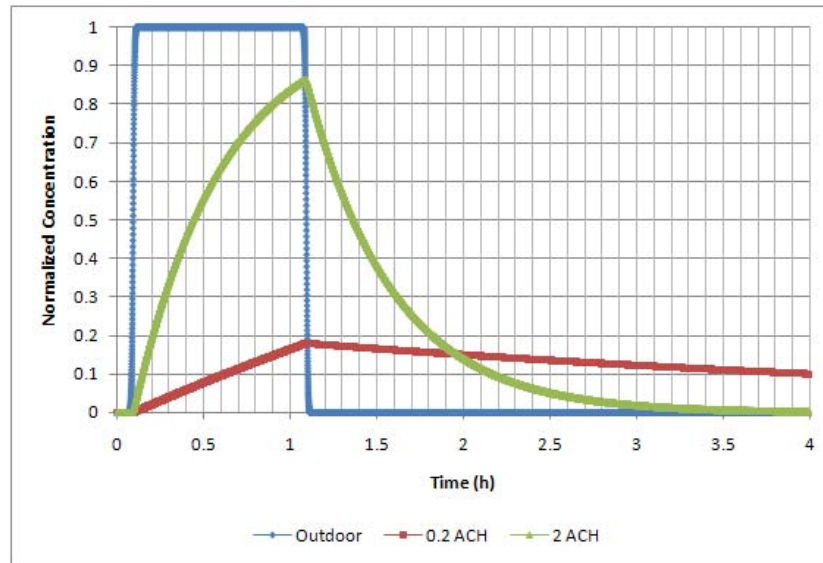
Figure 4-Chan 1-hour Release
