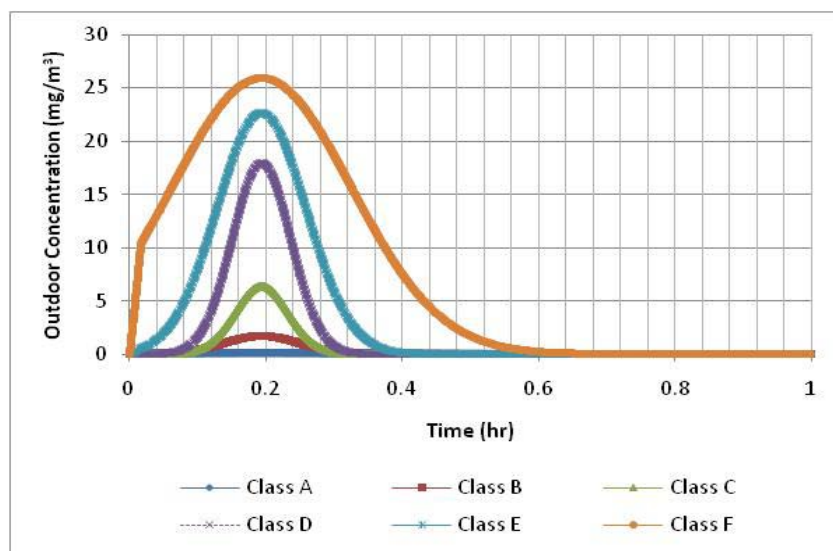
Figure 8-Stability Class Comparison
