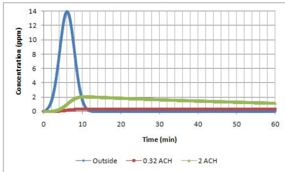
Figure 7-Sarin Validation Scenario
