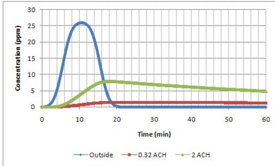
Figure 6-Chlorine Validation Scenario
