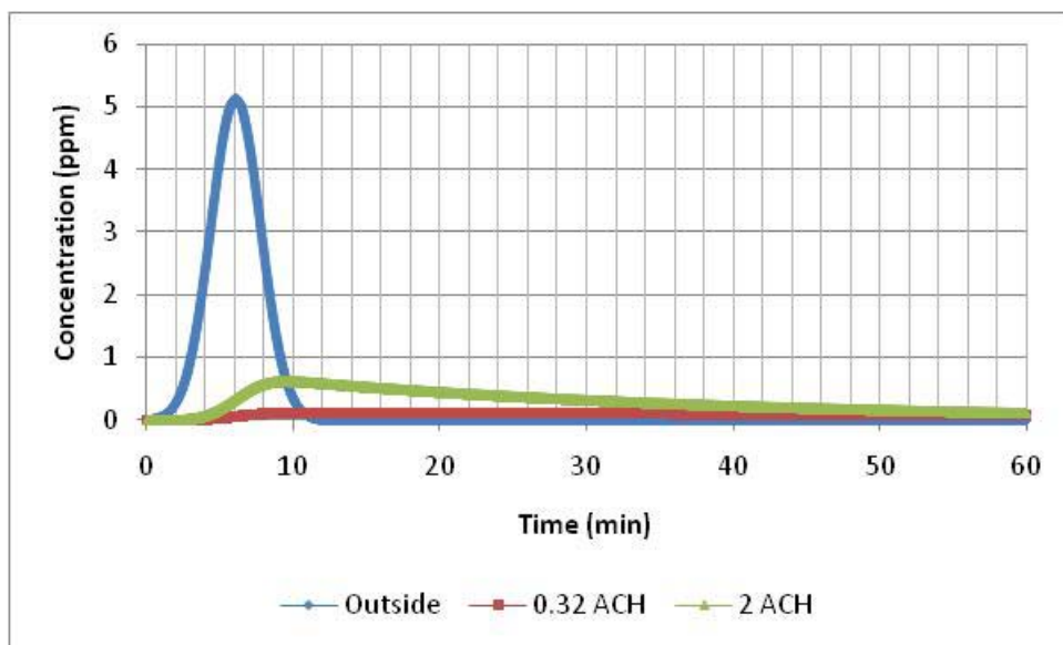
Figure 31- Model Sarin Concentration at Point (#2, 1 km)
