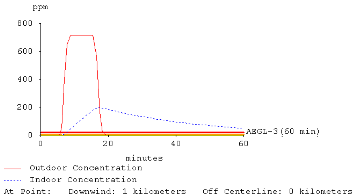
Figure 21- ALOHA Chlorine Concentration at Point (#2, 1km, 2 ACH)
