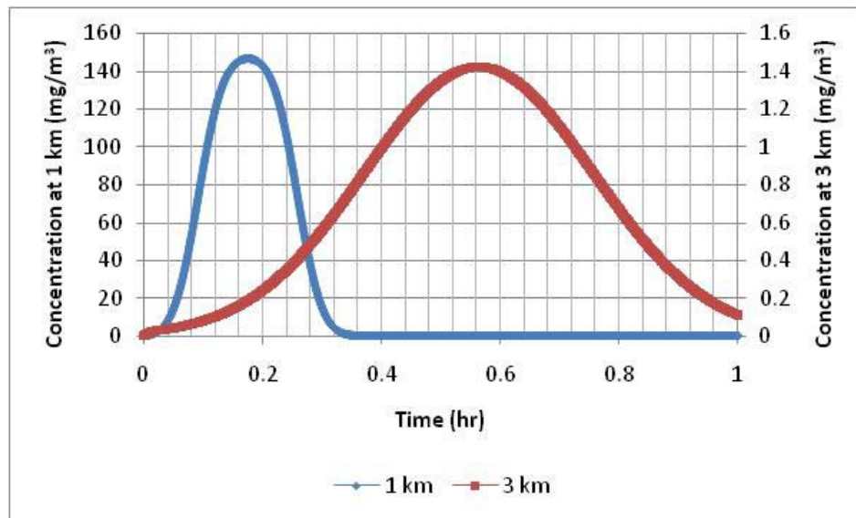
Figure 11-Distance Comparison
