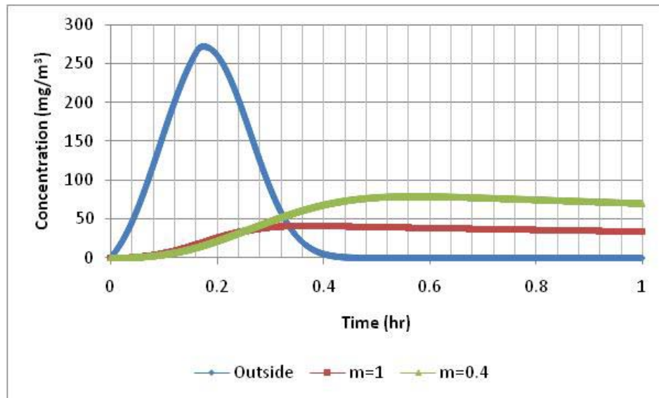
Figure 12-Well Mixing Comparison
