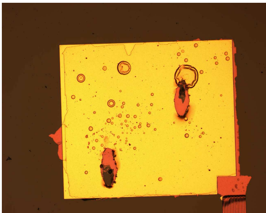
Figure B.22: Device 4.2 shows holes from low-power wire-bonding attempts.
