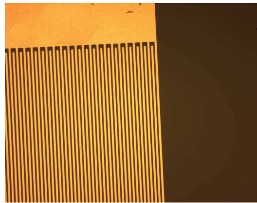
Figure B.33: Series 5 and 6 successful bondpad deposition (a) Sample 5.5.1L (b) Sample 6.4.1L shows undamaged fingers after bondpad fabrication.
