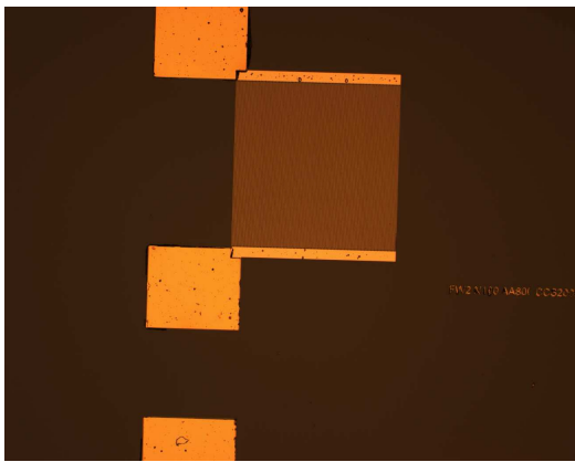
Figure B.33: Series 5 and 6 successful bondpad deposition (a) Sample 5.5.1L (b) Sample 6.4.1L shows undamaged fingers after bondpad fabrication.
