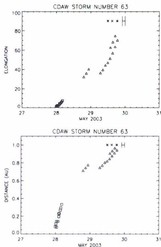
Figure 2. The 29–30 May 2003 ICME (Figure 1 (bottom)). CDAW storm 63 (top) elongation versus time and (bottom) distance versus time plots. See Figure 3. The symbols are as follows: squares, leading edge of CMEs in LASCO C2 and C3; triangles, leading edge of ICMEs in SMEI; asterisks, shock ATs at L1 at ACE or Wind (Shock Date and Time column of Table 2); crosses, SMEI aurora onset time (Aurora Date column of Table 2); vertical bars, storm onset and peak times ( Dst Date column of Table 2). The d – t data is used to calculate the arrival times of the ICME at 1 AU based on linear fits to the three separately tracked SMEI features; the two later ATs are given in Predicted 3-D column of Table 2.
