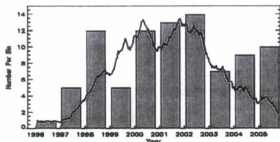
Figure 10. The yearly occurrence rate of the 88 CDAW storms. The black curve is the 180-day running average of daily sunspot numbers in arbitrary units. From Zhang et al. [2007a, 2007b].
