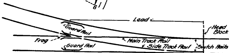
FIGURE 6-Arrangement of Turnout
