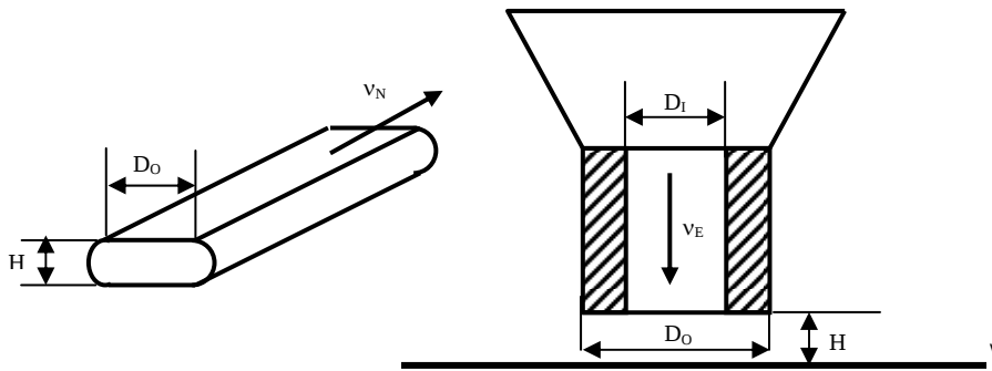
Figure 7. Schematic drawings showing the dimensions of the nozzle and slab shaped extrudate.
