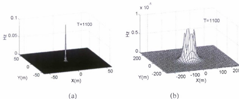
Figure 2.2. (a) Near-field mesh plot, (b) Far-field mesh plot.
