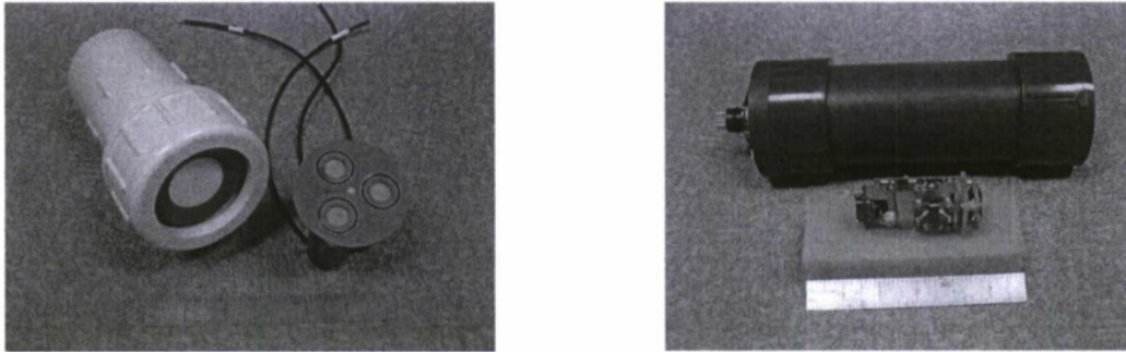
Figure 9: Electric (left) and magnetic (right) sensors.
