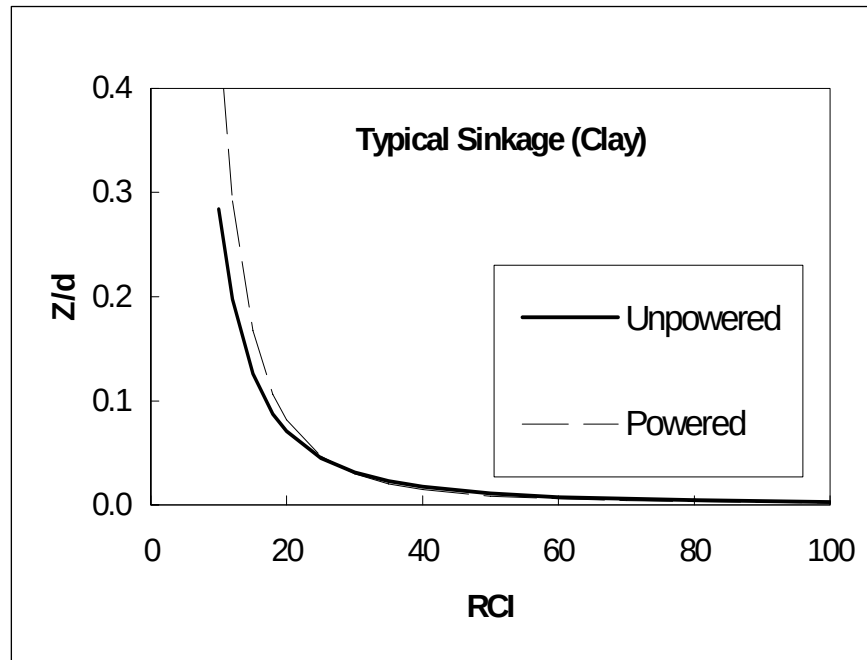
Figure C1. Sinkage of the HMMWV in clay based on the WES numeric.
