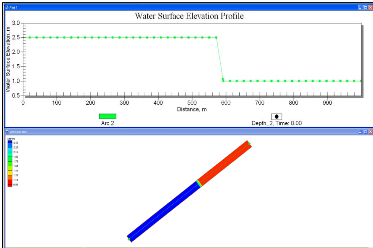
Figure 3. Water-surface elevation, 1.5-m drop.
