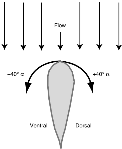
Fig. 3. Orientation of the flipper model in the wind tunnel as seen from above. Data were collected every 2^\circ as the model was rotated between +40 and -40 angle of attack ( \alpha ).
