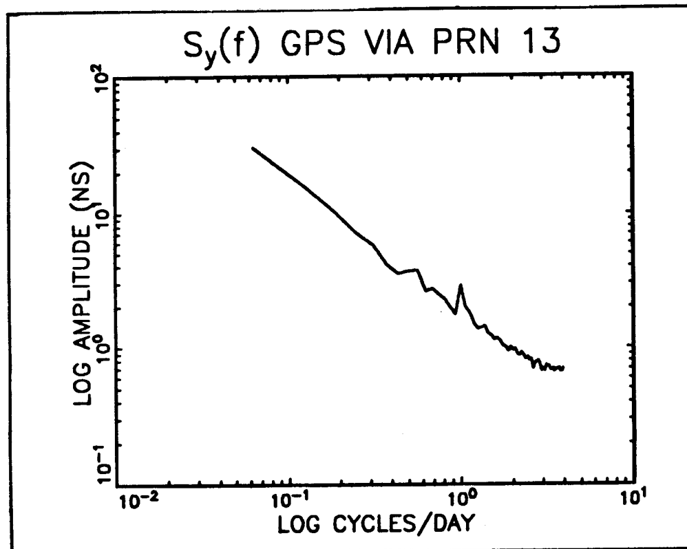
Figure 5: The Fourier transform of GPS minus Global UTC(NBS) from PRN 13 only has a significant diurnal variation. This is representative of the data via any individual SV.
