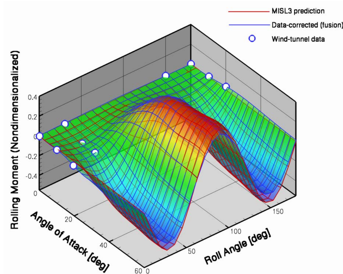
Figure 10: MISL3 and Experimental Rolling Moment Predictions.
